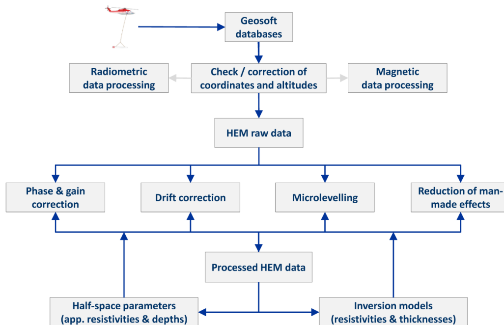
Figure 6.1: The advanced HEM data processing includes four principal steps: phase and gain correction, drift correction, microlevelling and reduction of man-made effects.
