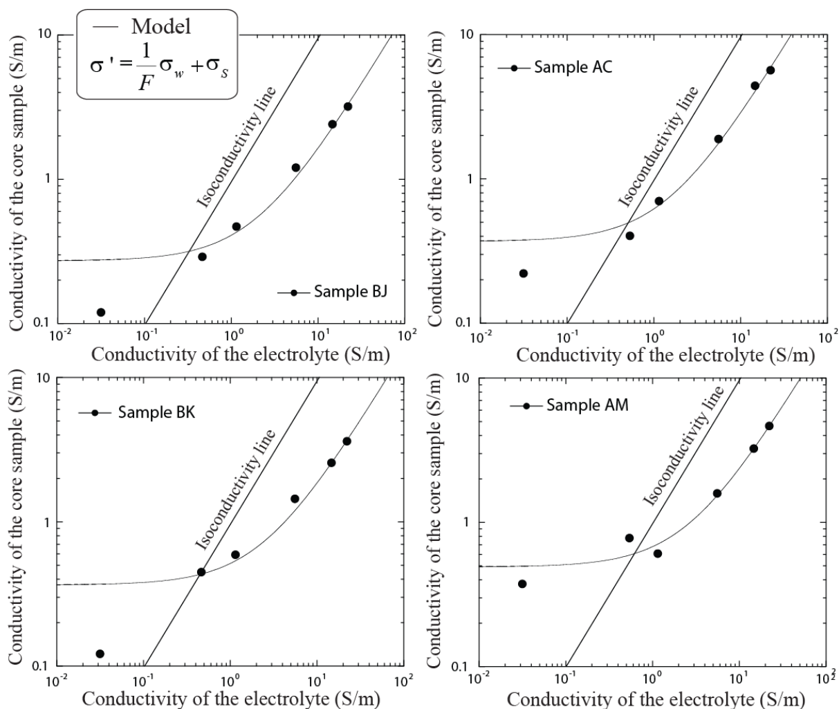
Figure 8.5 Fits of Equation 9.1 to bulk conductivity measurements of different samples saturated with known pore water conductivities. Note that axes are on log-scale, so the linear line of Figure 8.1 is curved in these plots.
