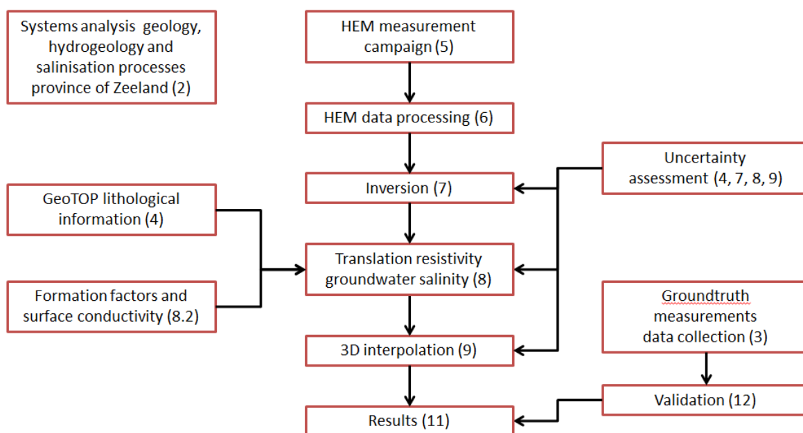
Figure 1.2 Procedural steps in the FRESHEM methodology, numbers between brackets refer to chapters in this report where these steps are further described.
