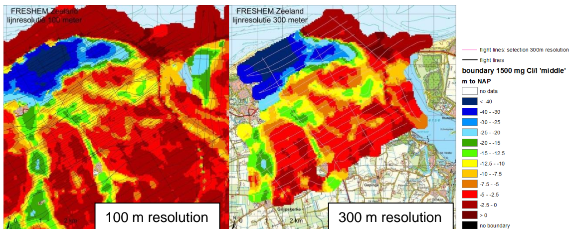
Figure 10.6 Flightline resolution: a. 100 metre between the flightlines (pink and black lines) and b. 300 metre between the flightlines (only pink lines) for the test area Walcheren.
