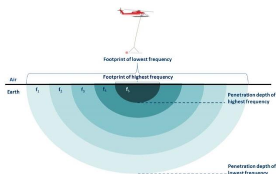
Figure 5.4: Footprint vs frequency of the HEM system.
