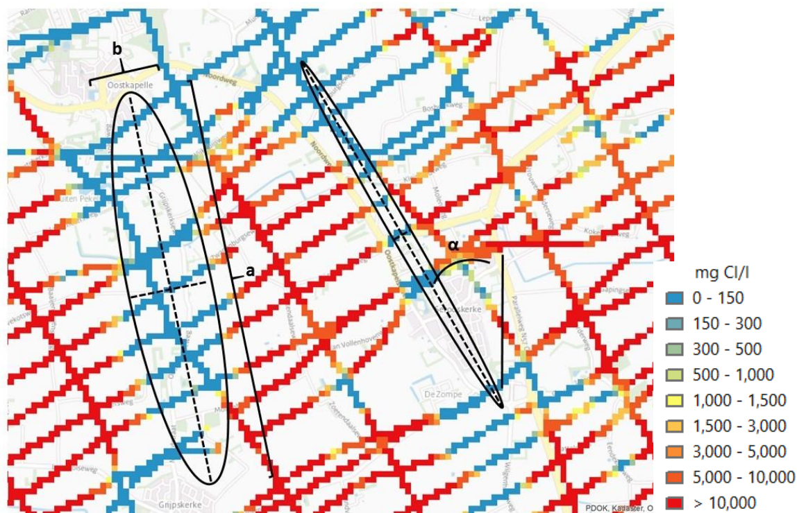
Figure 9.7: Visualisation of the parameters of the anisotropy ellipse, with p50 of 2D result at 6 m below NAP: \alpha angle of long axis, a length of long axis, b length of short axis.
