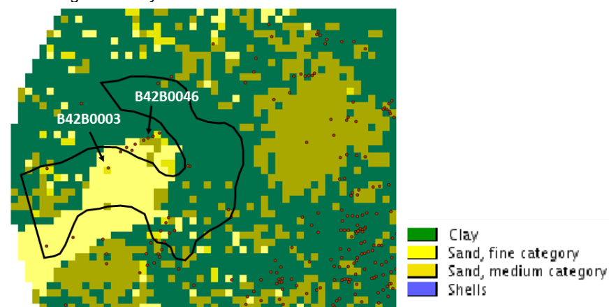
Figure 11.29 Interpretation of the high resistivity body, projected on GeoTOP lithological prediction at 19 m below NAP. Red dots are GeoTOP boreholes that at least reach the Naaldwijk Walcheren member, logs of two selected boreholes shown in Figure 11.30. See Figure 11.31 for the legend.
