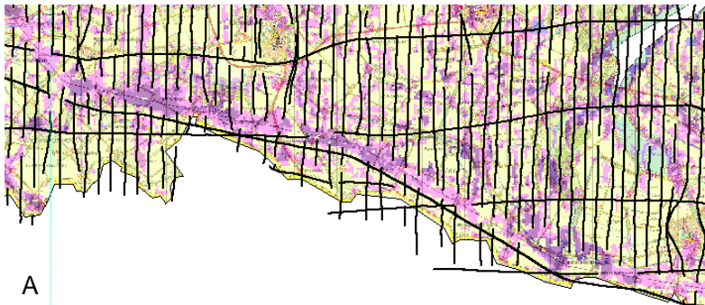
Figure 11.9 Uncertainty depth 1500 mg Cl/l boundary: difference depth 'low' and 'high' as % of depth 'middle'. For location (A) and legend, see Figure 11.8. Visualized are the flightlines and the no-data gaps in the flightlines. The uncertainty increases above the power line.
