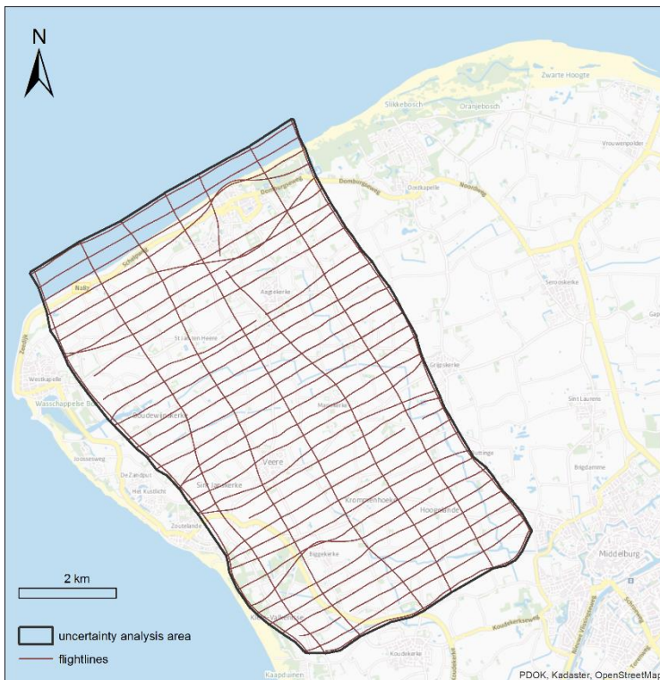
Figure 10.1: Area considered for the uncertainty analysis (black line), with the flightlines in this area (brown lines).
