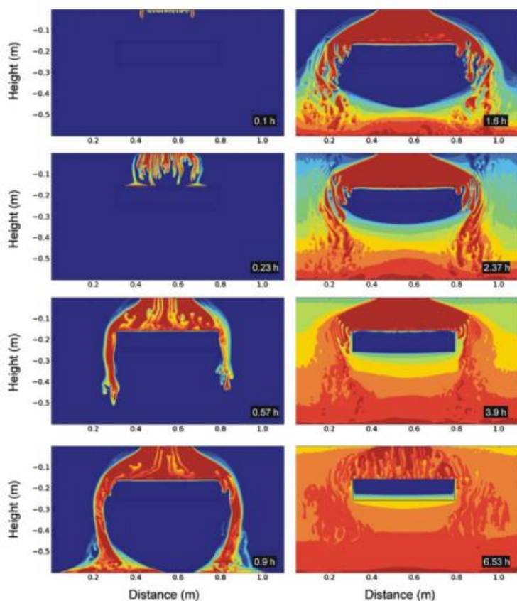
Figure 2.7: Numerical simulation of a laboratory experiment of free convection (from: Post en Simmons, 2009). In the middle of the model a low-permeable clay layer is present. The absolute speed of salinisation shown here is not representative for reality, however, the figures do illustrate the relative difference in speed of salinisation between the permeable section and the clay layer.
