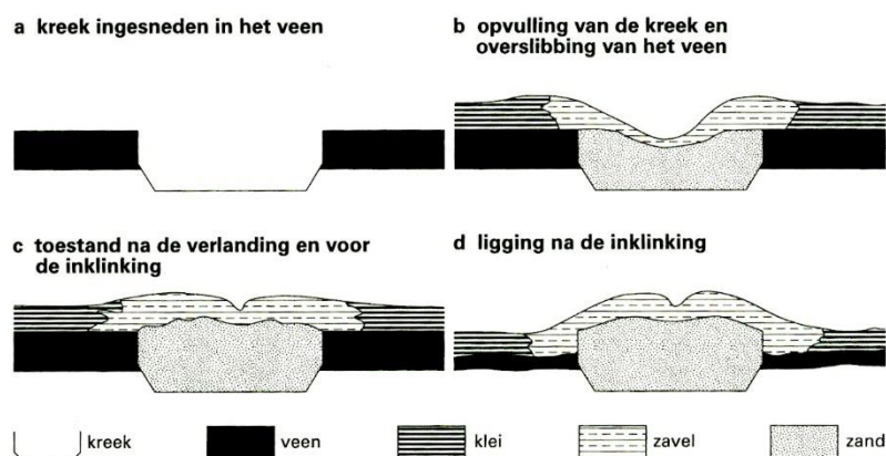
Figure 2.5: Development of a creek ridge (schematic). a) incision of a channel in underlying sediments; b and c) clay is deposited on the flats and sand fills the channel; d) a high creek ridge after drainage and settlement (naar Berendsen, 2000).
