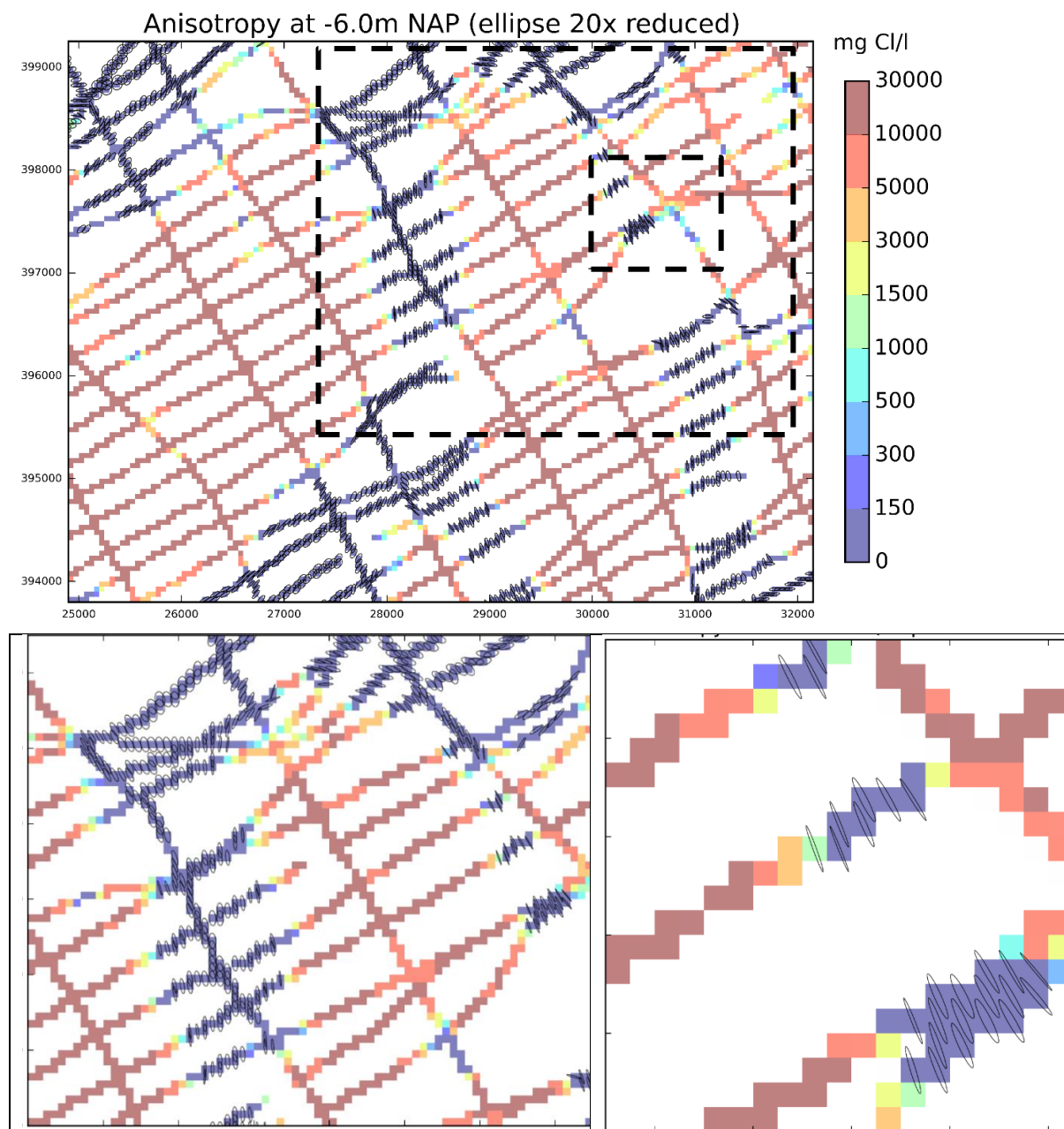
Figure 9.8: a) Anisotropy ellipses as determined directly from the 2D result, visualized at 6 m below NAP with p50 of 2D result, size of the ellipses is reduced 20 times. b) enlargement of area indicated in a), c) enlargement of smallest area indicated in a).
