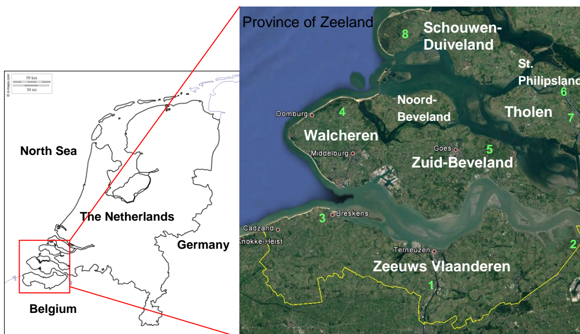
Figure 1.1 a. location of the Province of Zeeland in the Netherlands and b. the names of the islands and sub regions of Zeeland. The numbers in green correspond with the high resolution areas (section 1.1.3).
