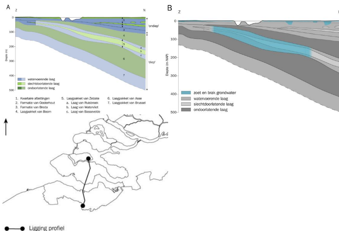
Figure 2.6: Regional cross section extending from Zeeuws-Vlaanderen (left) towards Zuid-Beveland (right). From: Goes en Vernes, 2000. REGIS Zeeland Deelrapport C: Zoet, brak en zout grondwater. In A, the green layers indicate the aquitards, whereas the blue layers indicate the aquifers. Names of the corresponding formations and member are also indicated. Below A the location of the transect can be seen. In B, blue denotes fresh and brackish water. The grey layers correspond to the aquifers and aquitards as indicated in A.
