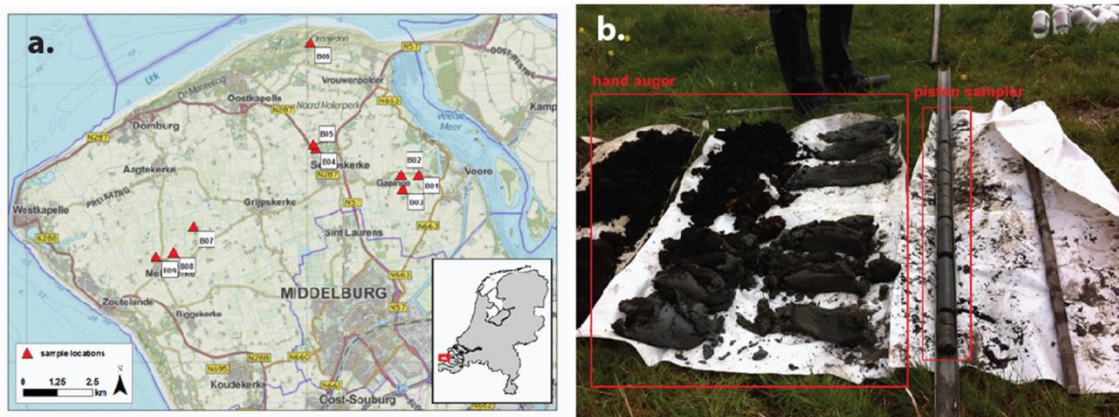
Figure 8.2 Sampling campaign: a) sample locations, and b) example of soil collection using hand auger and piston sampler.
