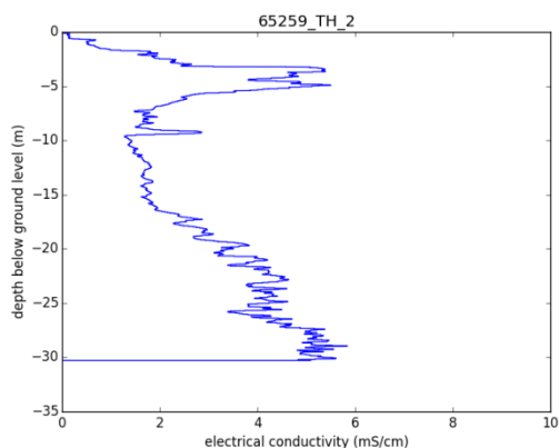
Figure 11.23: Cone penetration test at Tholen. In the upper 5 m the salinity increases, then decreases and finally increases again from ~16 m below ground level.
