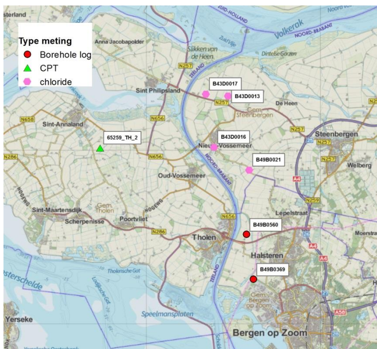
Figure 11.25: Overview of the different independent measurements around De Eendracht / Schelde-Rijnkanaal that support the presence of the inversions.
