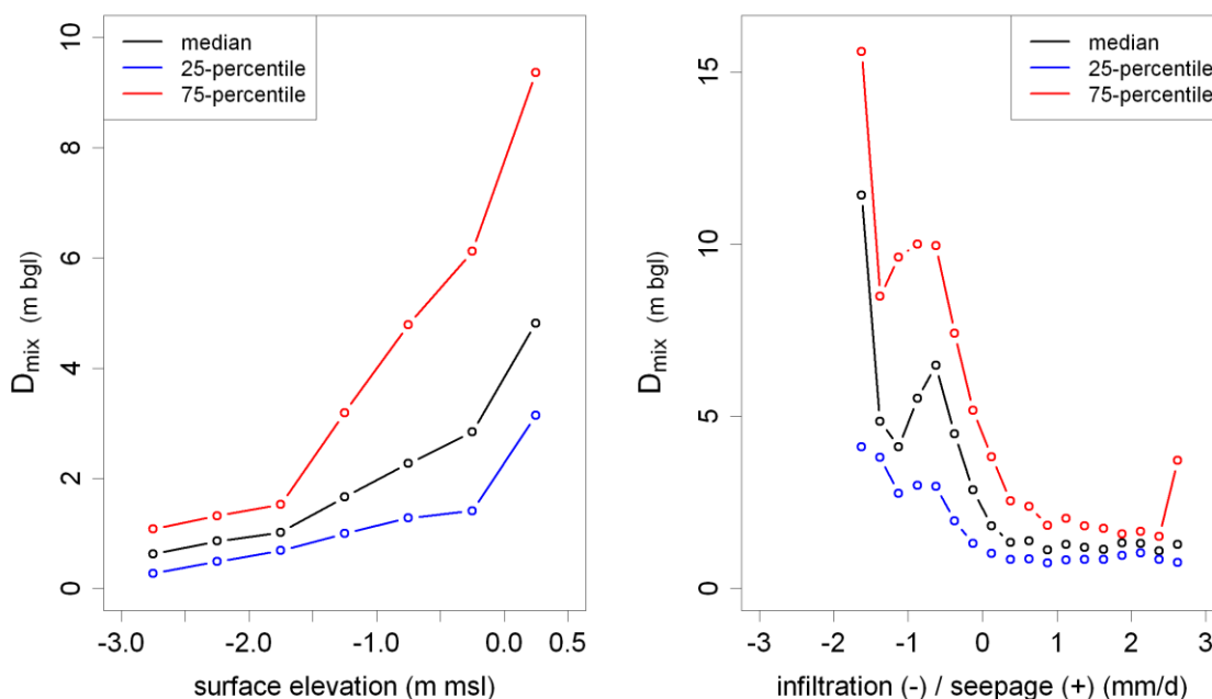
Figure 2.8 Relation of the middle of the fresh-saline interface ( D_{mix} ) derived from 84,300 HEM-measurements at Schouwen-Duiveland in 2009 with (a) Surface elevation (m MSL) and (b) Infiltration and seepage flux (mm/d). The 25-, 50- and 75-percentile of D_{mix} was determined and plotted for different classes of surface elevation and flux (dots represent middle of class) (De Louw, 2011).
