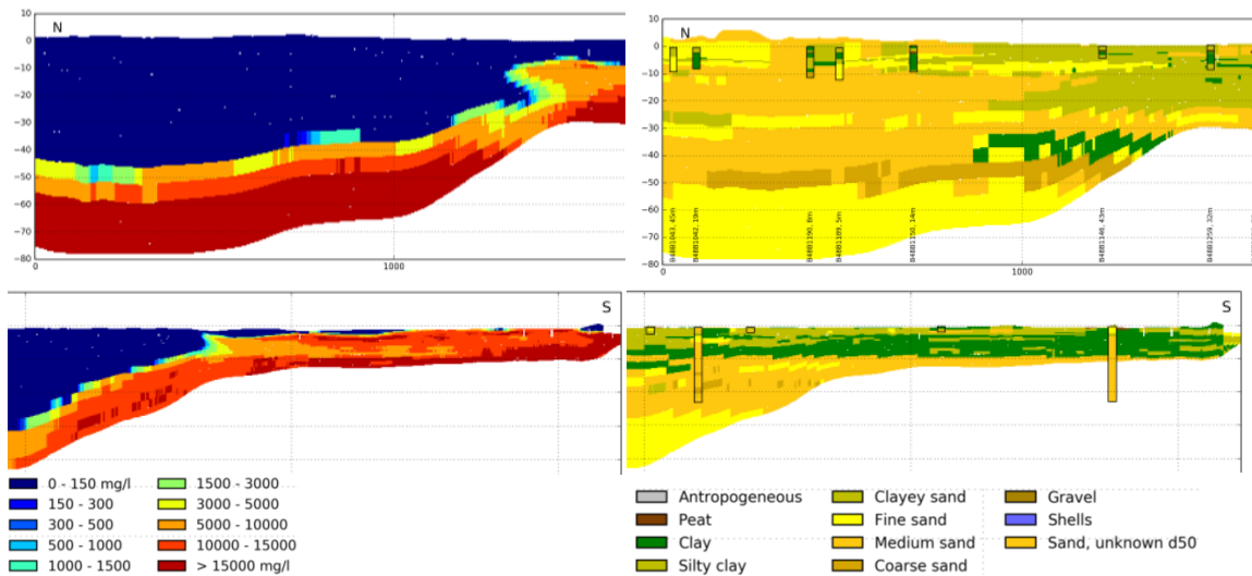
Figure 11.18: Inversions along the inland boundary of the dune areas of Oranjezon (Walcheren) (above) in flightline 109.9, and Schouwen-Duiveland (below) in flightline 126.9.
