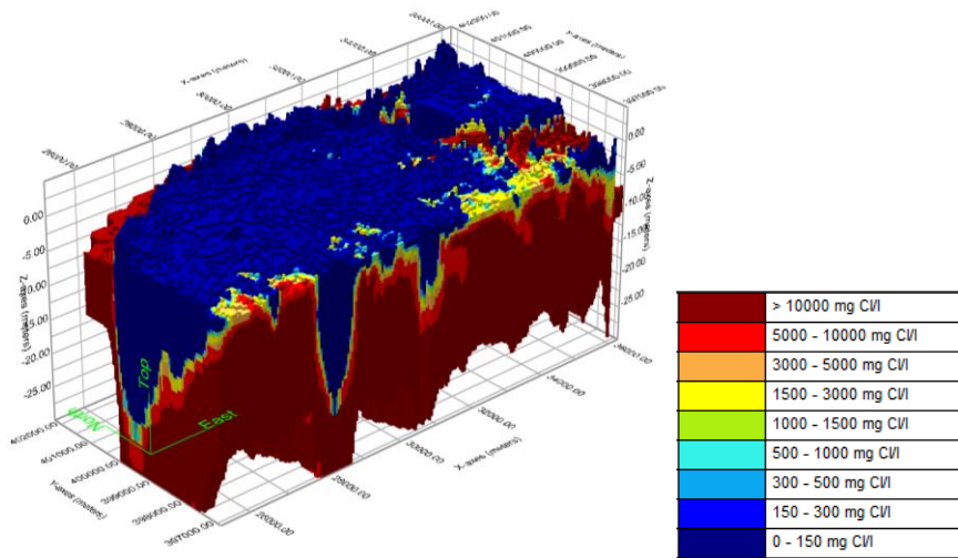
Figure 11.3 3D example FRESHEM 'middle' for part of Walcheren. West the dune area Oranjezon and in the south two sandy creek ridges near Serooskerke.
