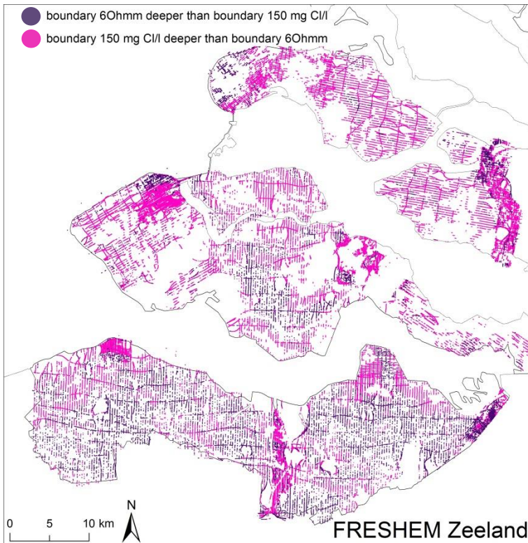
Figure 11.37 In pink the locations (measurement 2D result FRESHEM) where the 150 mg Cl/l boundary is deeper than the 6 \Omega m boundary. In purple the locations where the 6 \Omega m boundary is deeper than the 150 mg Cl/l boundary.
