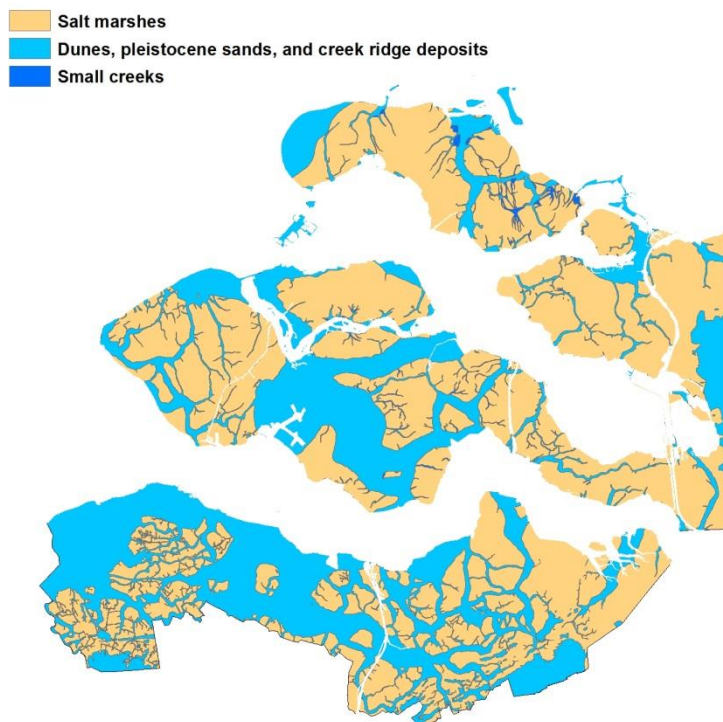
Figure 2.9: Types of deposits found at the surface: salt marshes, creek ridge deposits, small creeks, dunes, and Pleistocene sands. In general, fresh groundwater in the phreatic aquifer is found in the blue areas, whereas saline groundwater is found in the confining layer in the yellow areas.
