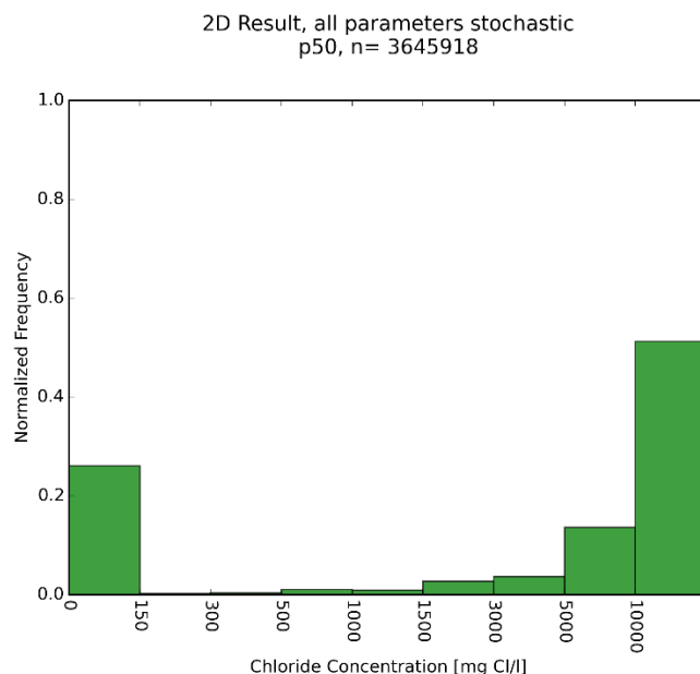
Figure 9.1: Histogram of the median value (p50) of chloride concentrations of the 2D result, for the area indicated in Figure 10.1.
