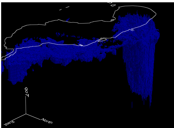
Figure 11.4 3D example showing only freshwater occurrence 'middle' for island Schouwen-Duiveland. Blue is fresh groundwater (<1500 mg Cl/l), visualized in iMOD. West (right) the dune area of Schouwen-Duiveland with a large freshwater lens.
