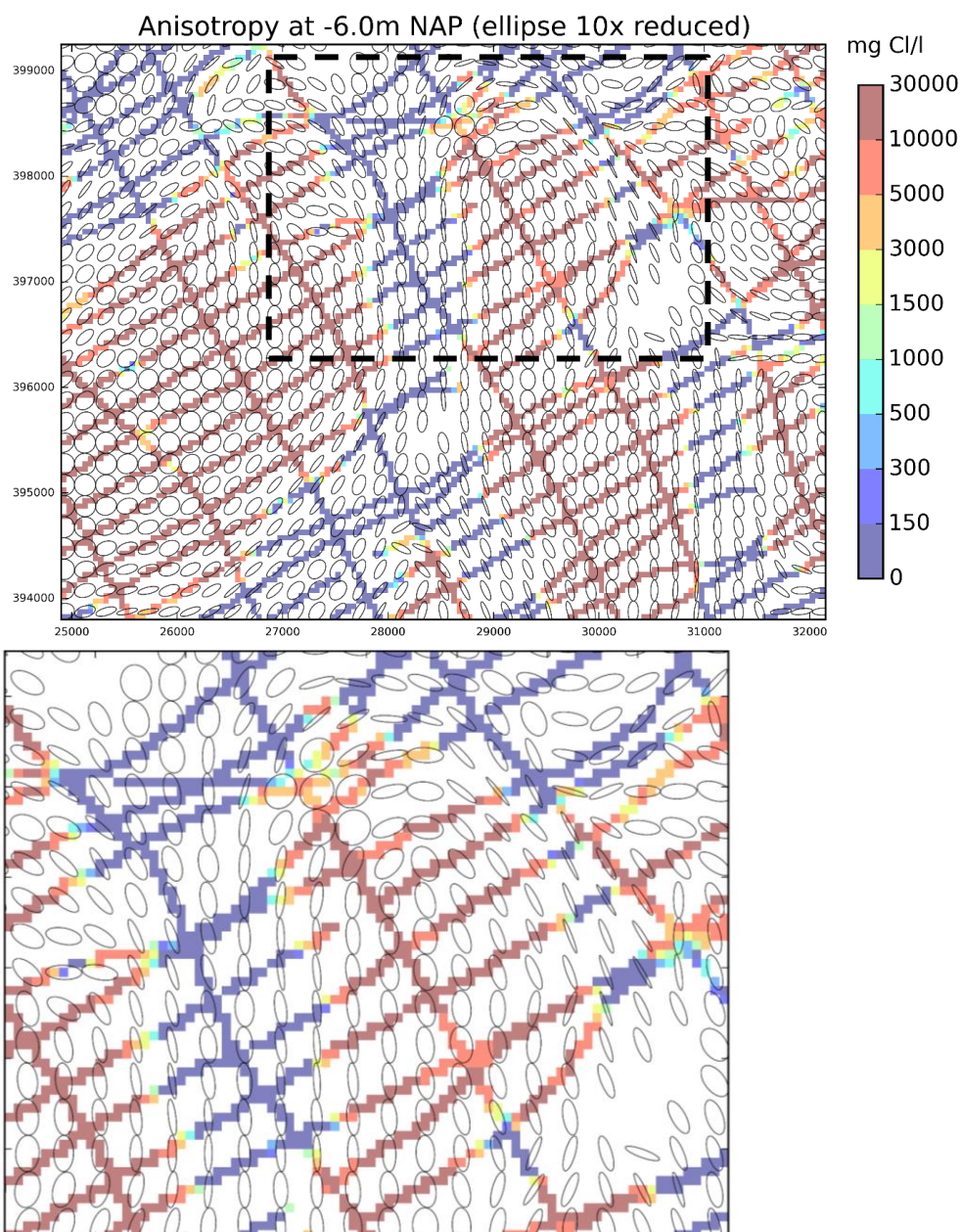
Figure 9.9: a) The LVA field, visualized at 6 m below NAP with p_{50} of 2D result, size of the ellipses is reduced 10x. b) enlargement of area indicated in a)
