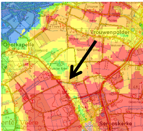
Figure 11.13 Depth 1500 mg Cl/l boundary FRESHEM Zeeland 'middle'. For legend and location see Figure 11.11.
