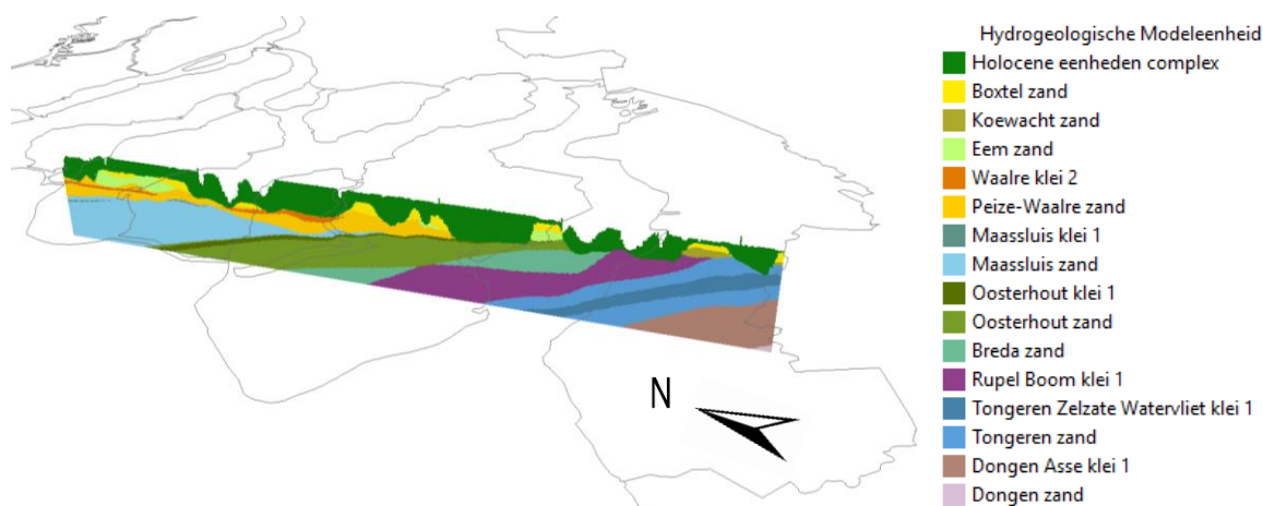
Figure 2.1: Birds-eye-view from the southwest on the deeper subsurface of Zeeland (TNO-GSN, in press). Displayed is a North-South cross-section with hydrogeological units to a depth of 100m below Dutch Ordnance Datum (NAP).
