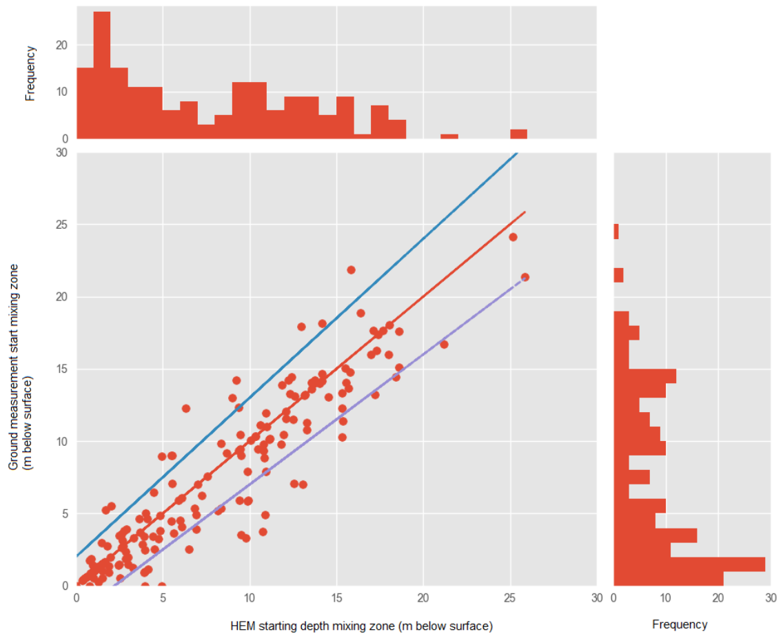
Figure 12.11 Scatterplot of HEM starting depth of the fresh salt-mixing zone versus ground measurement starting depth. The red line indicates the 1:1 relationship. The blue line gives an upper bound estimate on the starting depth of the mixing zone, and the purple line gives a lower bound estimate. Marginal histograms at the top and right show the distribution of the starting depths: many starting depths are shallow.
