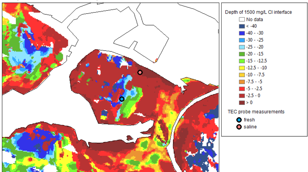
Figure 12.12 Example of two TEC probe measurements in St. Philipsland, Zeeland, overlaid on the depth below surface of the fresh-saline interface (defined by 1500 mg/L).
