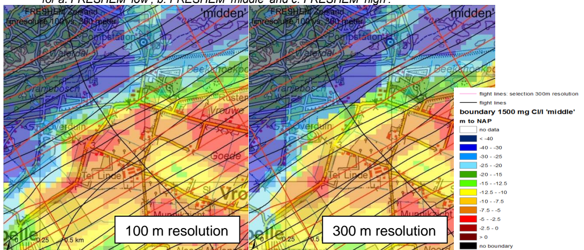
Figure 10.8 Flightline resolution: a. 100 metre between the flightlines (red and black lines) and b. 300 metre between the flightlines (only red lines). The high flightline resolution results in the mapping of the saline seepage area near the dunes (in the middle of the figures).
