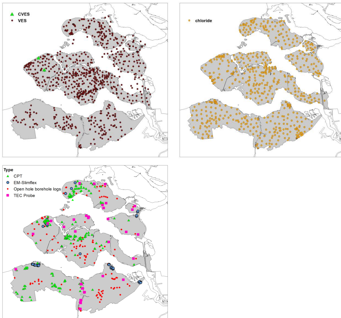
Figure 3.6: Overview of different types of ground truth measurements.
