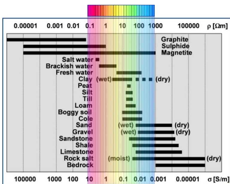
Figure 5.1: Typical electrical conductivities (resistivities) for diverse materials vs. with helicopter-borne electromagnetics detectable range (colours).
