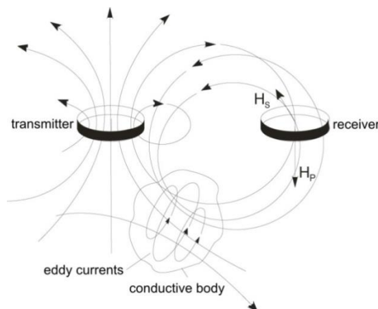
Figure 5.3: Transmitter and receiver EM concept (after Knödel et al. 2007).
