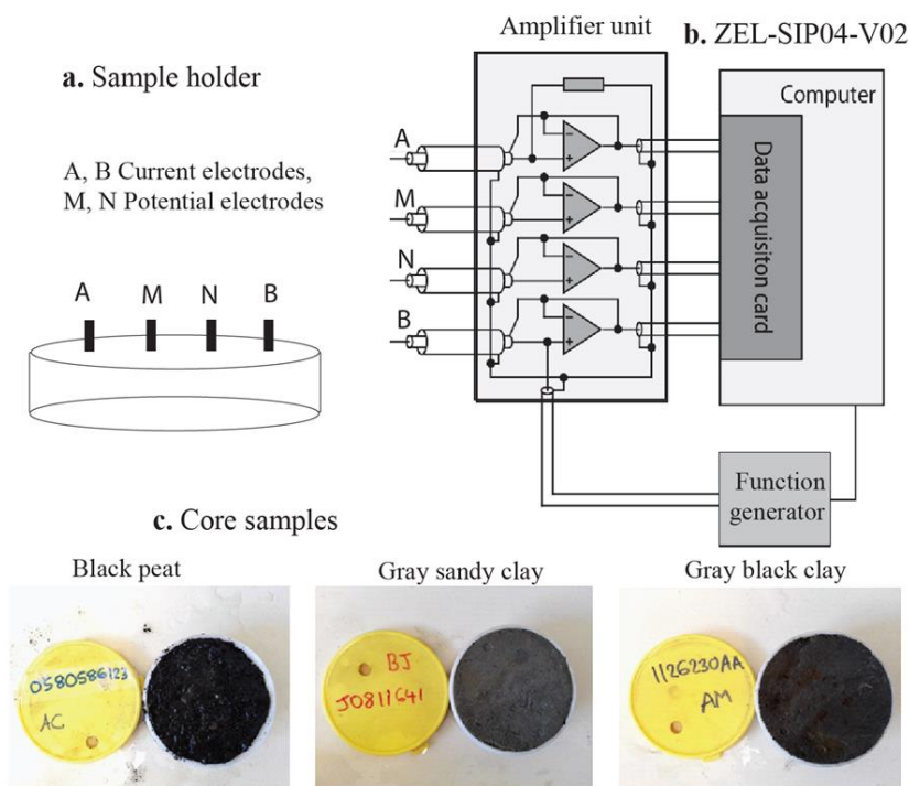
Figure 8.3 Measurement setup for conductivity measurements
