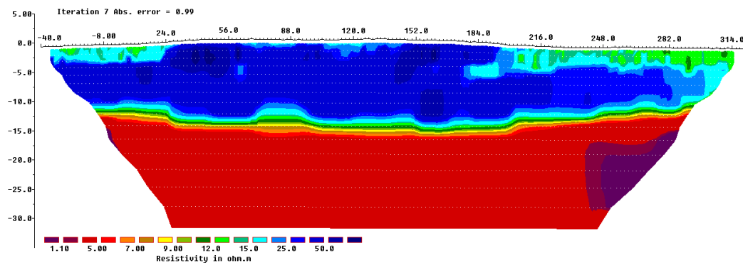
Figure 11.19: Inversion result of a CVES measurement along a creek ridge south of Grijpskerke (Walcheren).
