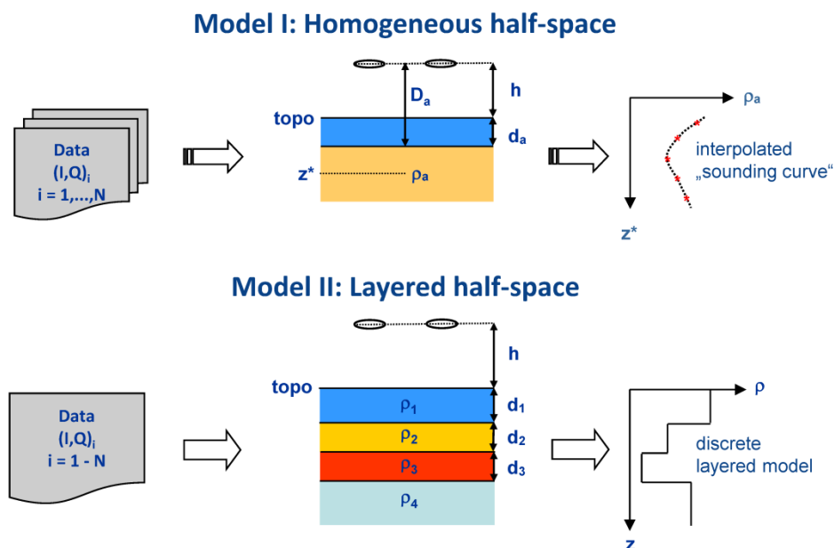
Figure 7.1: HEM data inversion based on homogeneous and layered half-space models.
