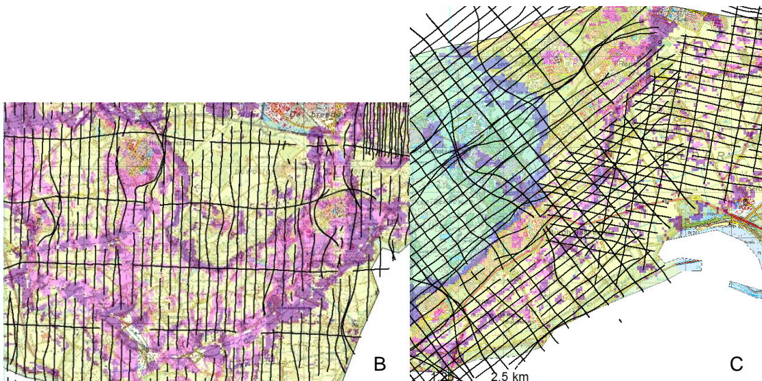
Figure 11.10 Uncertainty depth 1500 mg Cl/l boundary: difference depth 'low' and 'high' as % of depth 'middle'. Visualized are the flightlines and the no-data gaps in the flightlines. For location (B and C) and legend, see Figure 11.8. Figure a. Zuid-Beveland: the uncertainty increases above power lines, roads, rail ways and build-up areas. Figure b. Schouwen-Duiveland: the uncertainty increases and the horizontal boundary of the fresh groundwater lens.
