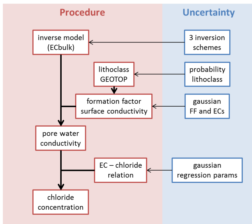
Figure 8.7: Overview of procedure and uncertainty approach
