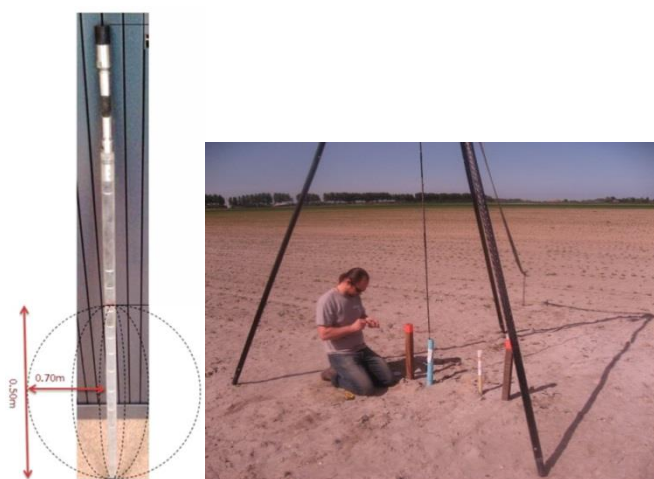
Figure 3.4: EM-Slimflex tool (left) and measurement (right)
