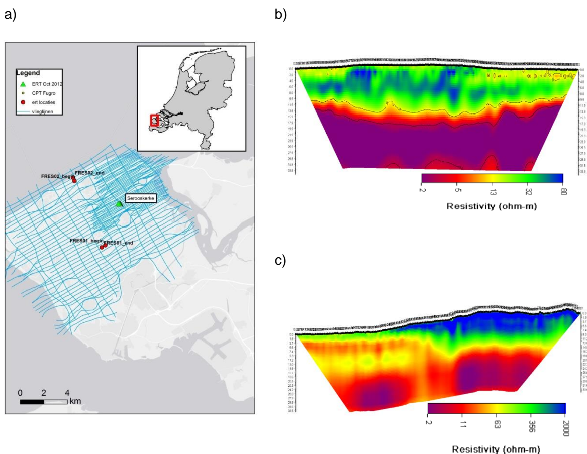
Figure 7.2: a) Map showing the locations of the two ERT profiles FRES01 and FRES02 and the flightlines. The additions ‘_begin’ and ‘_end’ indicate respectively the beginning and end of the two ERT profiles. b) ERT result for FRES01, c) ERT result for FRES02. Note the difference in color scale between b) and c).
