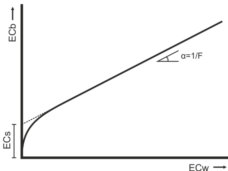
Figure 8.1 Relationship of bulk conductivity ( EC_b ) and pore water conductivity ( EC_w ). The tangent of the linear part is the reciprocal of the formation factor. The linear part crosses the y-axis at maximum surface conductivity ( EC_s )
