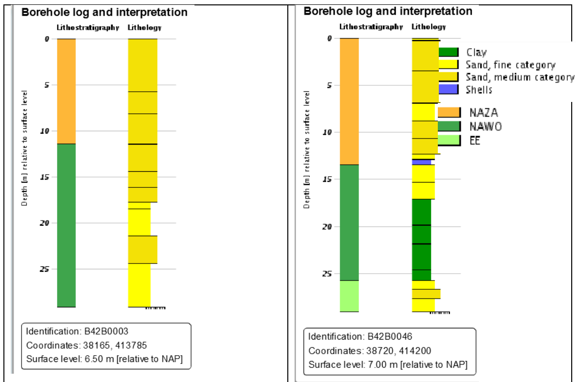
Figure 11.30 Two boreholes showing the transition from the sand to clay at 10 metre below NAP.
