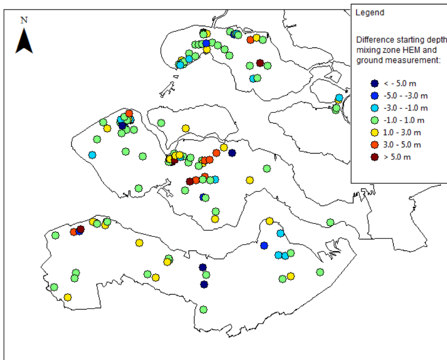
Figure 12.10 Validation result difference starting depth of fresh-saline mixing zone. Positive values indicate larger value of the mixing zone starting depth in the 3D FRESHEM result compared to the ground measurement.
