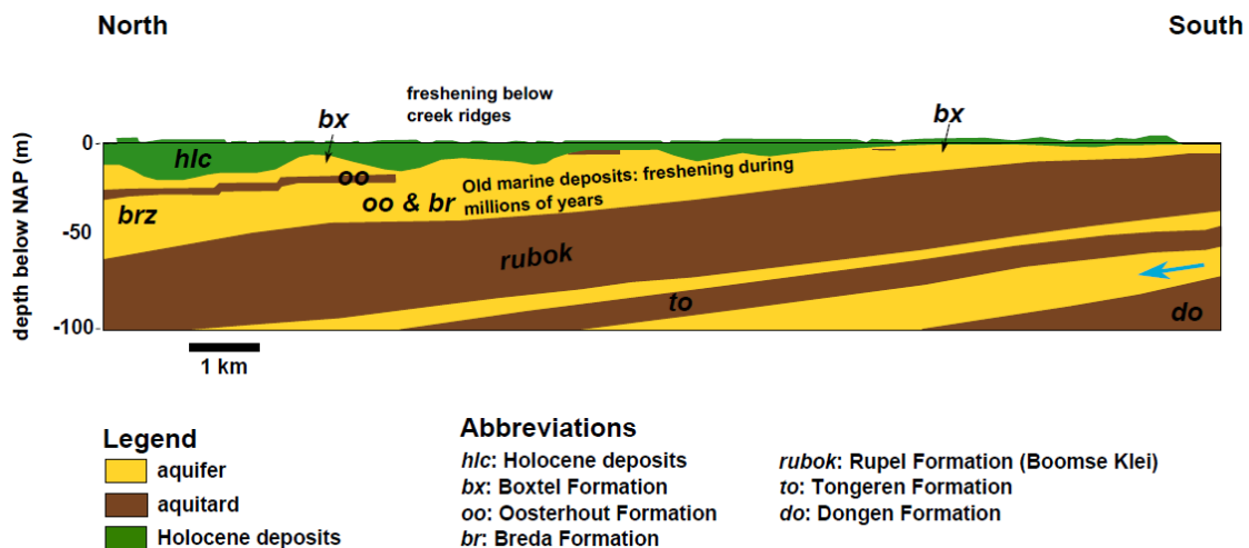
Figure 11.26: Inversions and hydrogeology in Zeeuws-Vlaanderen. See Figure 11.15 for the locations of the hydrogeological cross sections.
