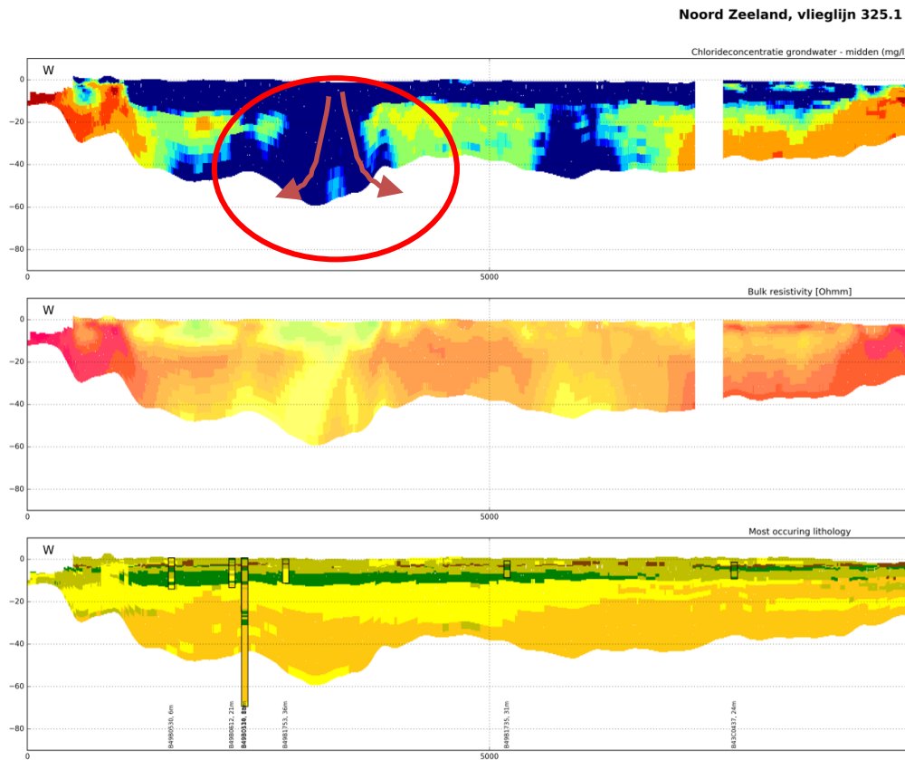
Figure 11.32 Chloride concentration, resistivity and GeoTOP lithology of part of line 325.1, see Figure 11.31 for the legend.
