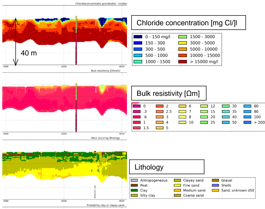
Figure 11.35: example (flightline 11.1 Midden Zeeland) of the mapping of fresh groundwater lenses in FRESHEM with a thickness of several metre (a) where the bulk resistivity remains below 6 Ωm (b) in areas with clay (c).
