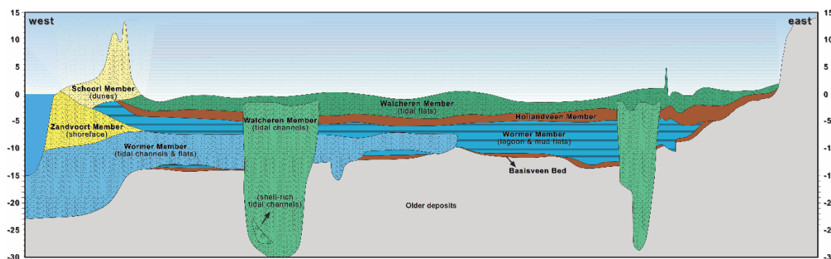
Figure 2.3: Conceptual West-East cross-section through Zeeland of holocene units (Stafleu et al. 2011).
