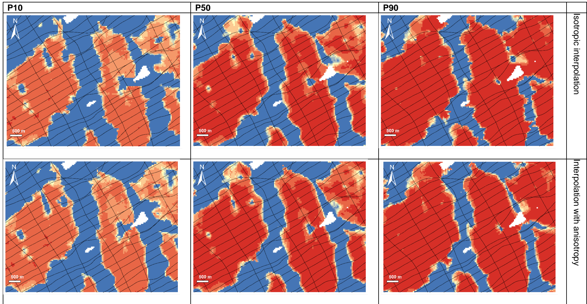
Figure 9.12: Depth slices at 6 metre below NAP. A comparison between the P10, P50 and P90 of the 3D model using isotropic and anisotropic indicator kriging. The area of interest is indicated in Figure 9.5
