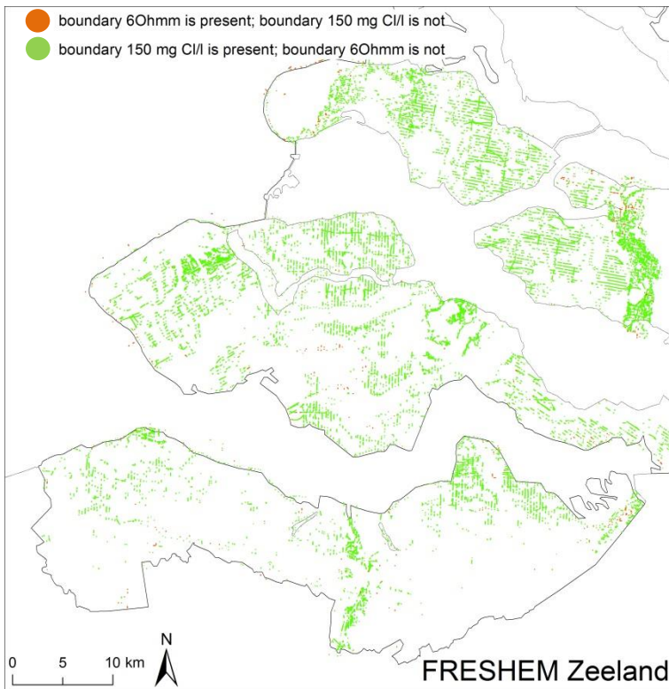
Figure 11.36 In green the locations (measurement 2D result FRESHEM) where the 150 mg Cl/l boundary is present and the 6 \Omega m boundary is not present. In orange the locations where the 6 \Omega m boundary is present and the 150 mg Cl/l boundary is not present.
