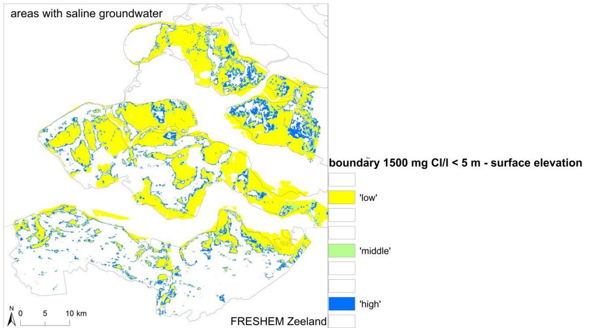
Figure 11.7 Areas in Zeeland with more less than 5 metre fresh (<1500 mg Cl/l) groundwater for 'low', 'middle' and 'high'.
