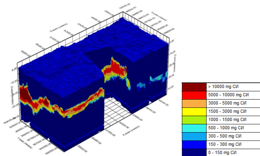
Figure 11.2 3D Example FRESHEM 'middle' for part of Zeeuws Vlaanderen.
