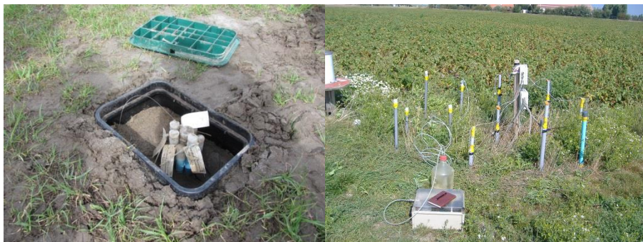
Figure 3.5: Chloride analyses of piezometre.
