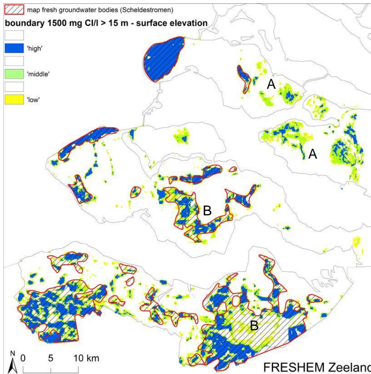
Figure 11.14 Areas in Zeeland with more than 15 metre fresh (<1500 mg Cl/l) groundwater for 'low', 'middle' and 'high' combined with the map 'fresh groundwater bodies' from Waterboard Scheldestromen.
