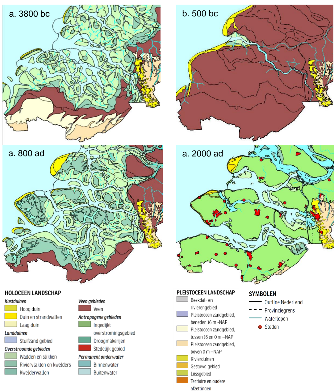
Figure 2.4: Palaeogeographical maps of Zeeland, from Vos & De Vries (2013).
