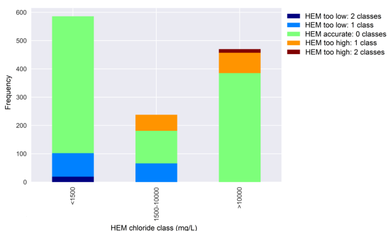
Figure 12.4 Validation result for chloride classes fresh, brackish and saline for FRESHEM result 'middle', per chloride class, absolute numbers.
