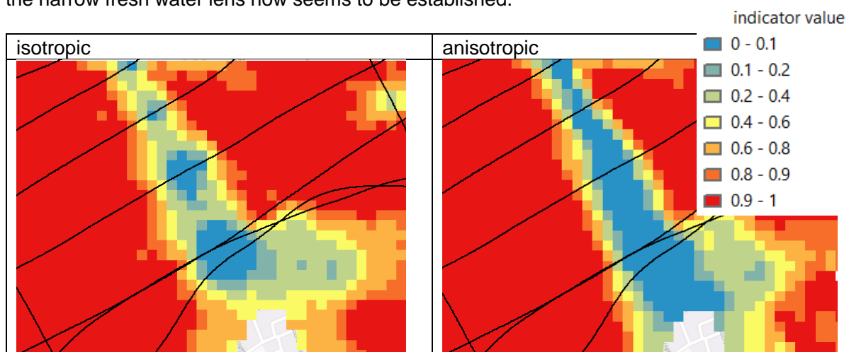
Figure 9.11: Interpolation result for the 1500 mg Cl/l indicator for interpolation with isotropic (left) and anisotropic neighbourhood and variogram (right). Black lines indicate flightlines.
