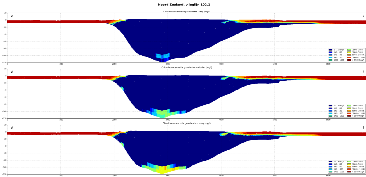
Figure 8.10: 25 th , 50 th and 75 th percentile chloride concentration (top, middle, bottom) for flightline 102.1 (Noord Zeeland)
