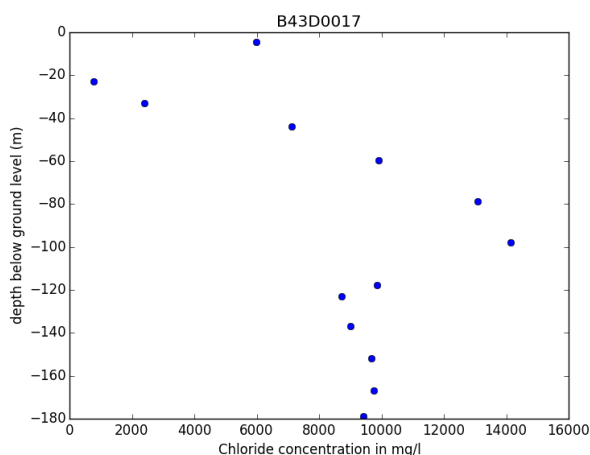
Figure 11.22: Chloride concentration of piezometre B43D0017, West of De Eendracht / Schelde Rijnkanaal. The upper filter shows brackish/saline groundwater, the filter below (21 m below ground level) is fresh. In this area also piezometre B430013, B430016, and B430021 (Figure 11.25) indicate fresh groundwater below saline groundwater in the FRESHEM result.
