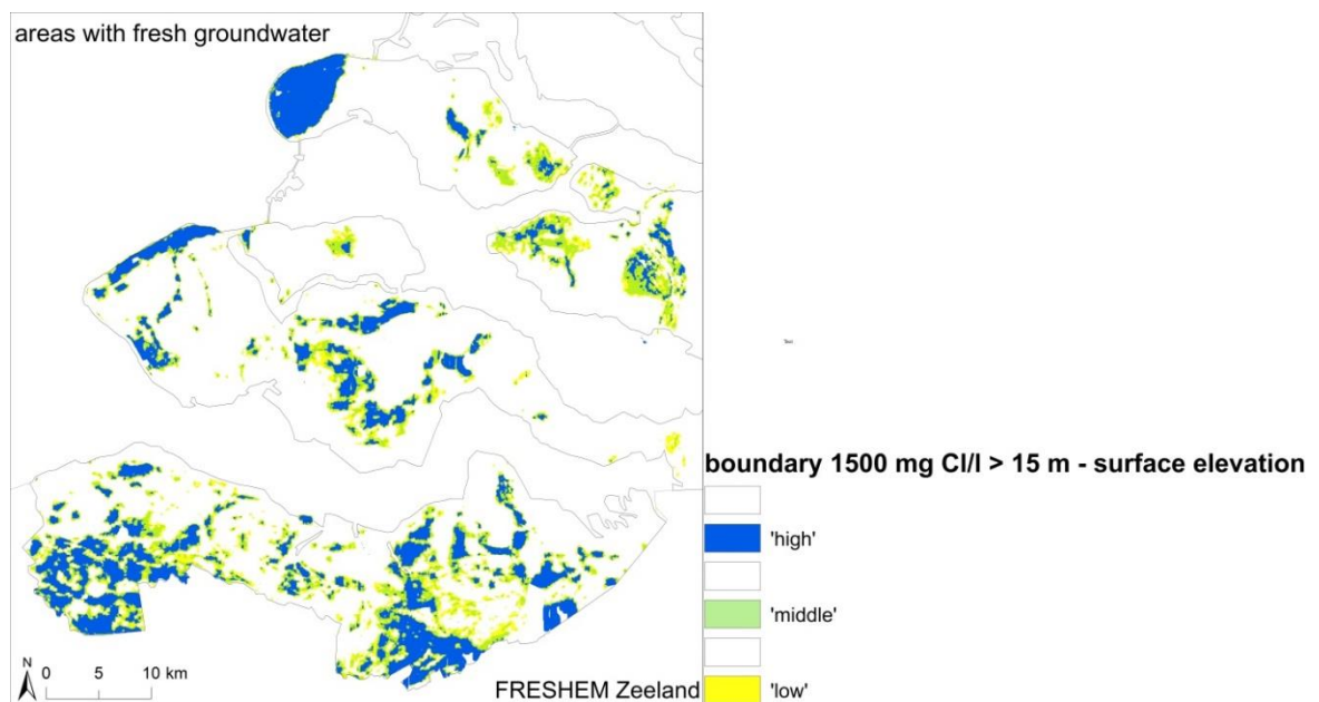
Figure 11.6: Areas in Zeeland with more than 15 metre fresh (<1500 mg Cl/l) groundwater for 'low', 'middle' and 'high'.
