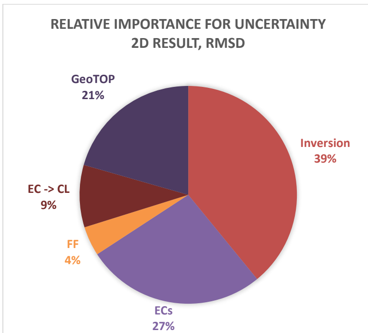
Figure 10.3: Pie charts of: a) the mean and b) the RMSD, of the difference between p10 and p90 for the different stochastic variables that are used to calculate the 2D result.
