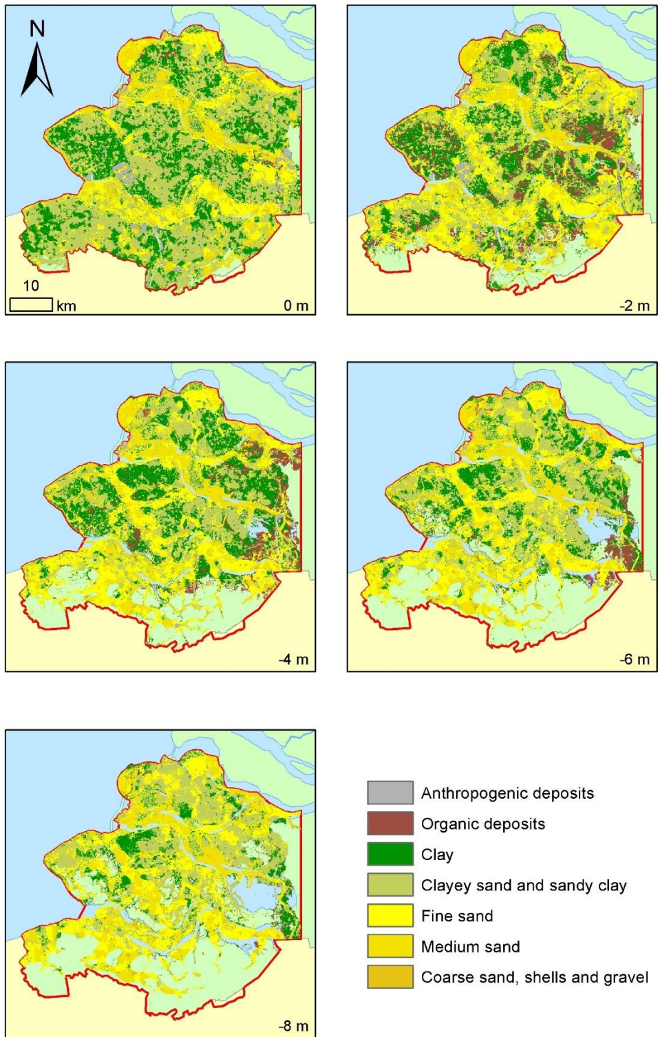
Figure 4.3: Horizontal slices through the lithofacies model at particular depths below Dutch Ordnance Datum revealing the position of tidal channels in the Walcheren Member (from Stafleu et al., 2011)
