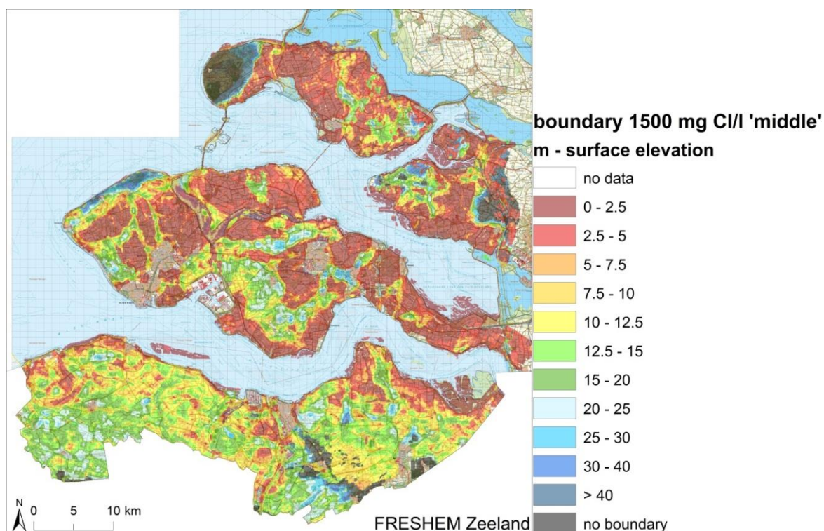
Figure 11.5 Depth of the 1500 mg Cl/l 'middle' boundary relative to surface elevation.
