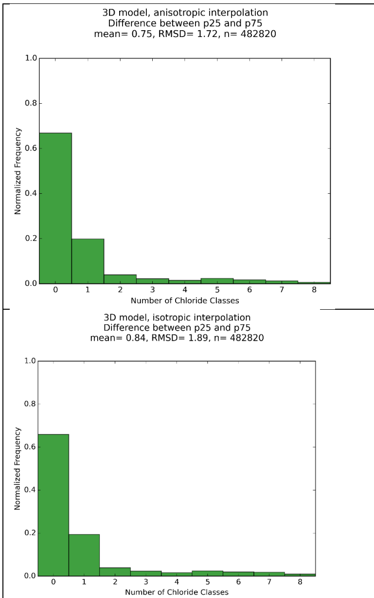
Figure 9.13: Uncertainty of the FRESHEM dataset expressed as the difference between the p25 and the p75 of the chloride concentration, for a) the 2D result, b) the 3D model as calculated with anisotropic interpolation, c) the 3D model as calculated with 'normal' isotropic interpolation
