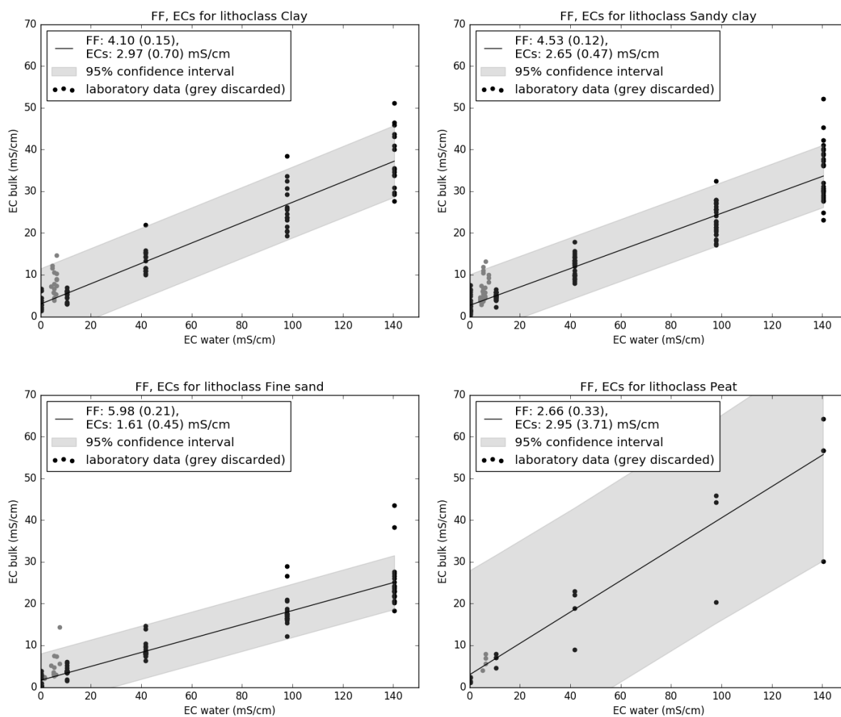
Figure 8.6 Results of derivation of formation factor FF and surface conductivity ECs per lithoclass.
