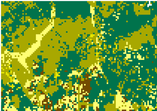
Figure 11.34: Lithological prediction from GeoTOP at 6.75 m below NAP shows a clay rich area at the same location where fresh water lens is relatively small. See Figure 11.31 for the legend.
