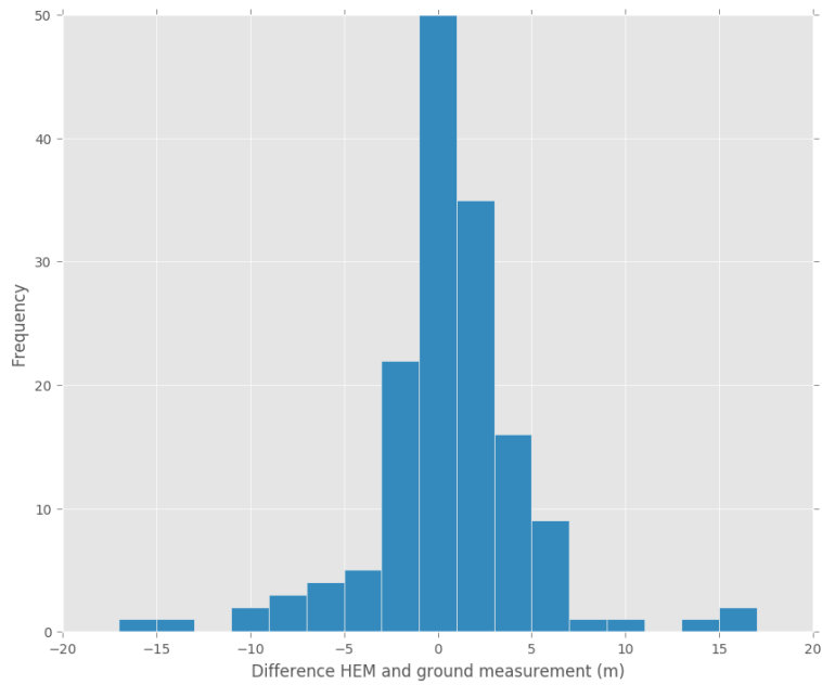
Figure 12.9 Histogram of the difference between the fresh-saline mixing zone thickness as determined from the 3D FRESHEM result, and from the ground measurements. Positive values indicate larger value of the mixing zone thickness in the 3D FRESHEM result compared to the ground measurement.
