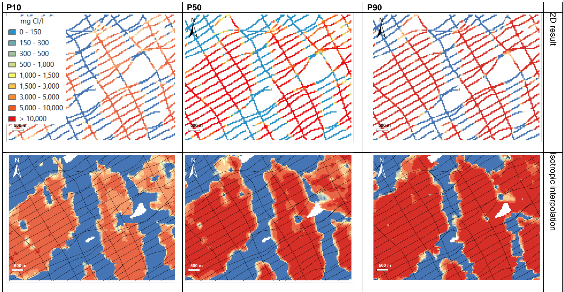
Figure 9.6: Depth slices at 6 metre below NAP. P10, P50 and P90 are shown for the 2D result and a 3D model using isotropic indicator kriging. The area of interest is indicated in Figure 9.5, black lines indicate flightlines.
