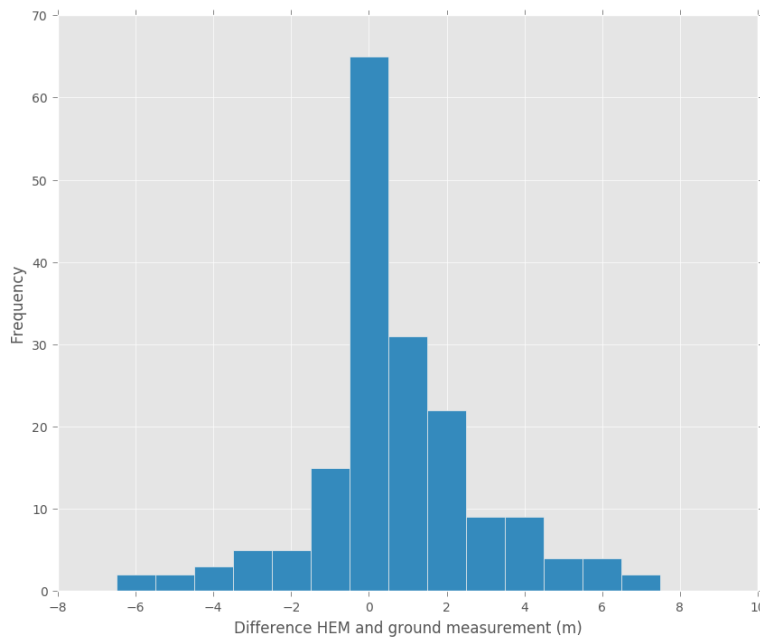
Figure 12.8 Histogram of the difference between the starting depth of the fresh-saline mixing zone as determined from the 3D FRESHEM result, and from the ground measurements. Positive values indicate larger value of the starting depth in the 3D FRESHEM result compared to the ground measurement.
