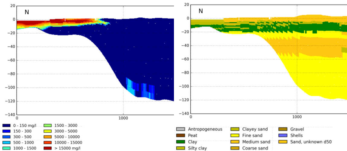
Figure 11.16: Inversion along the coast in flightline 128.9, perpendicular to the coast of Schouwen-Duiveland.
