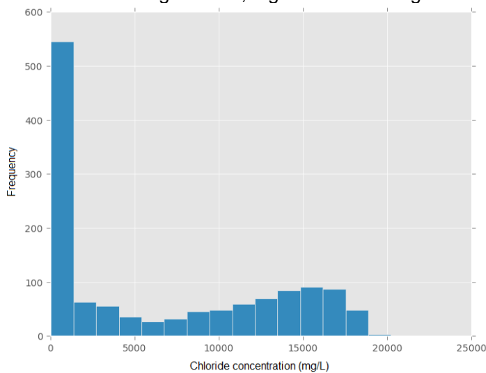
Figure 12.1 Histogram of chloride concentrations (median per well screen).
