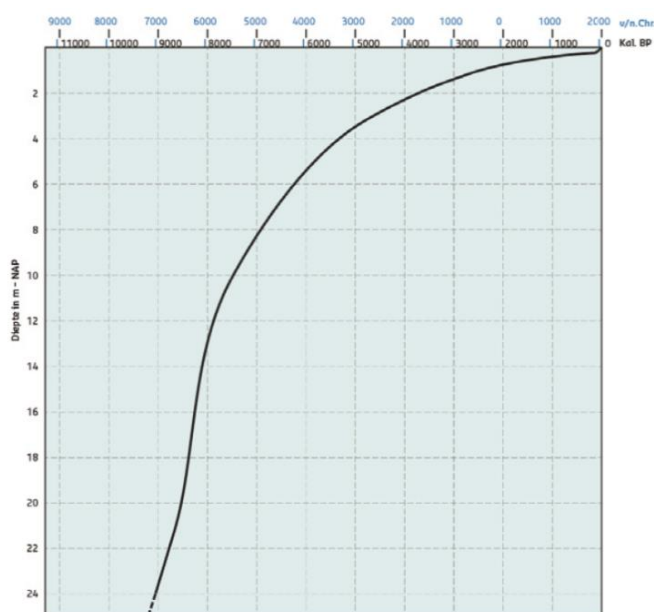
Figure 2.2: Sea level curve for the western Netherlands (from Vos & De Vries 2013).
