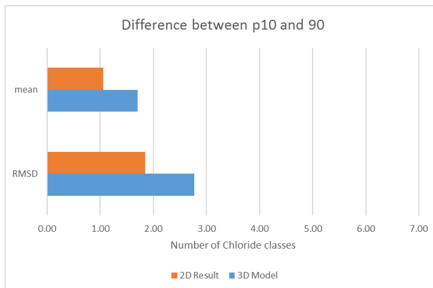
Figure 10.5: Mean and RMSD of the difference between p_{10} and p_{90} for the 2D result and the 3D model. 33% (mean) or 38% (RMSD) of the total uncertainty of the 3D model can be attributed to the spatial uncertainty added by interpolation.
