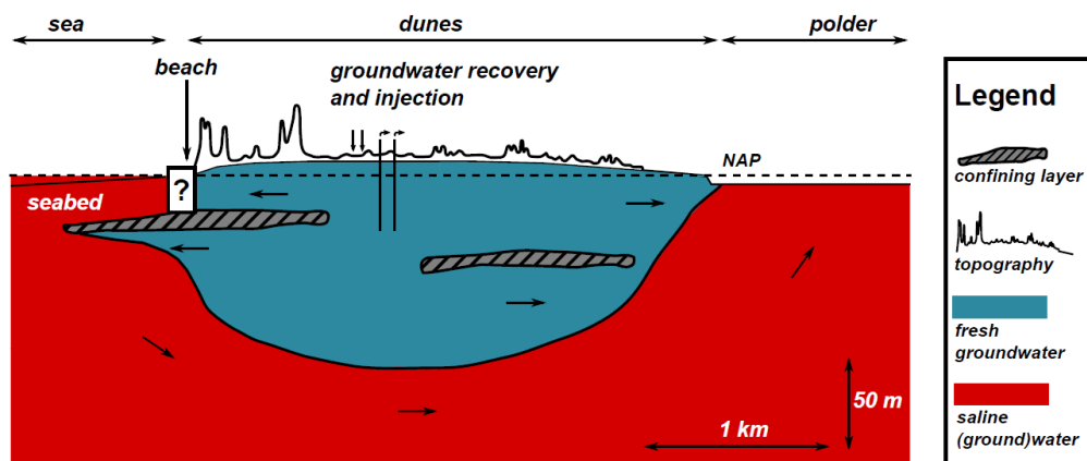
Figure 11.17: Concept of the groundwater salinity distribution along the Dutch coast (Pauw et al., 2017). Below the beach the groundwater salinity has been omitted and marked with a '?'. Saline groundwater also comprised brackish groundwater is this concept.
