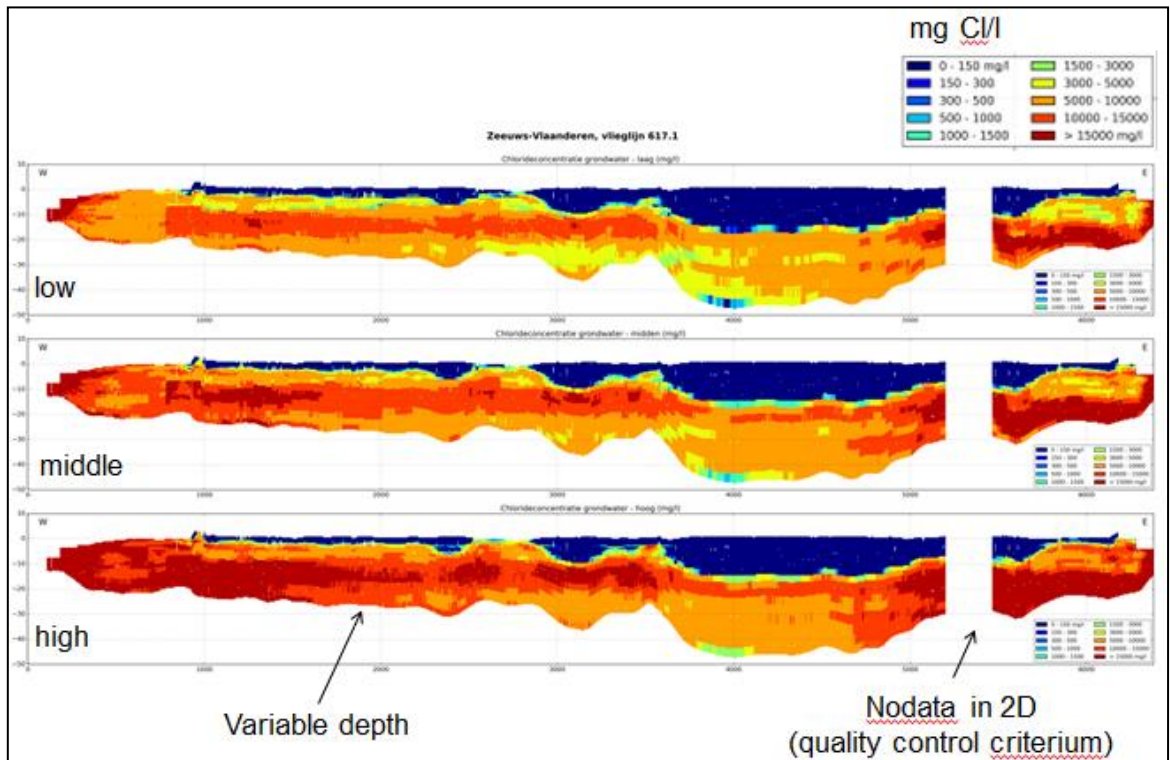
Figure 11.1 Example chloride concentration along the flightlines for 'low', 'middle' and 'high'.
