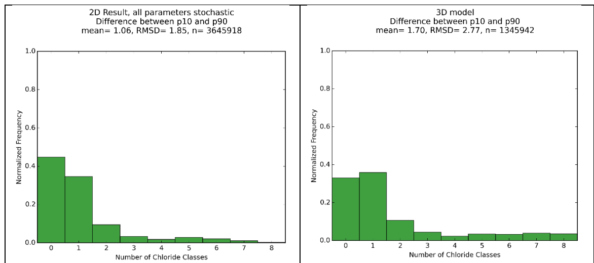
Figure 10.4: Histograms of p_{10} , p_{50} , p_{90} and number of classes difference between p_{10} and p_{90} , for 2D result and 3D model.
