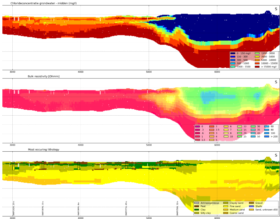
Figure 11.31 Chloride concentration, resistivity and GeoTOP lithology of part of line 431.1
