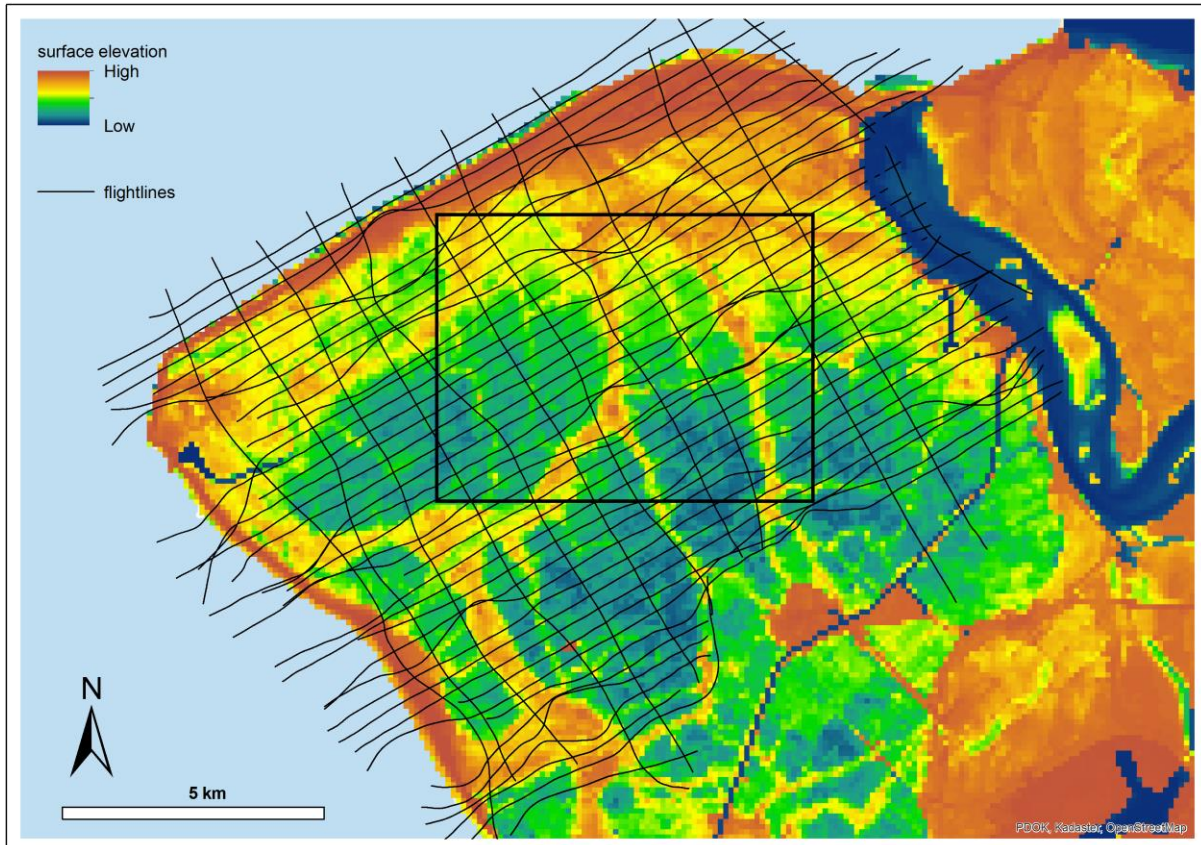
Figure 9.5: The surface elevation on Walcheren shows the elevated creek ridge morphology where elongated fresh water bodies are present. Flightlines are of set 169, that have been used for the anisotropy analysis in this section. The black box indicates the area of interest in this section.
