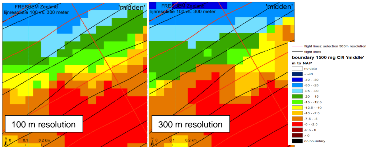
Figure 10.9 Flightline resolution: a. 100 metre (red and black lines) and b. 300 metre between the flightlines (only red lines). The high flightline resolution results in the mapping of the sw-ne freshwater lens.
