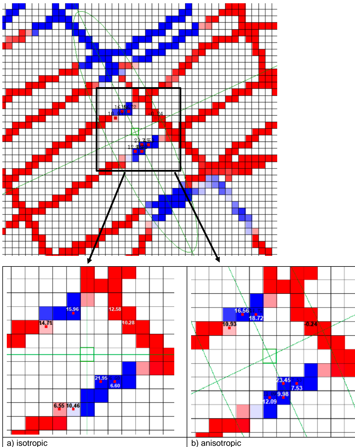
Figure 9.10: Effects of isotropic vs. anisotropic neighborhood and variogram on data selection and Kriging weights. a) isotropic, b) anisotropic.
