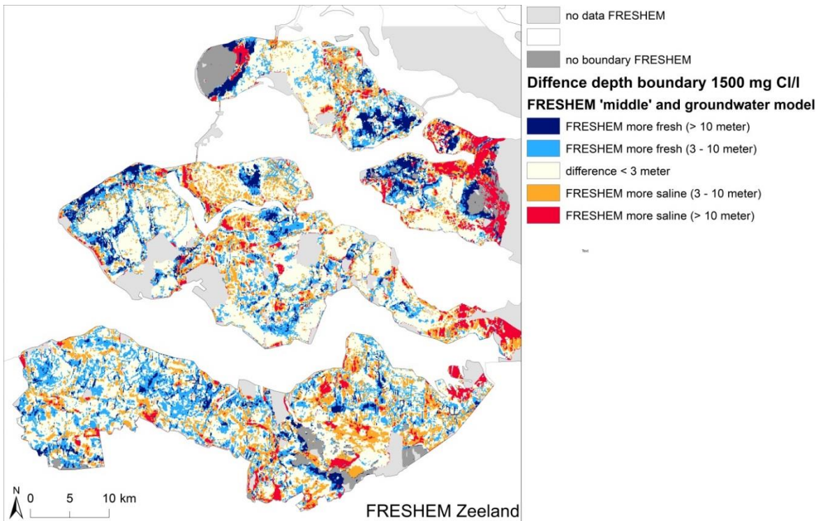
Figure 11.12 Difference in depth 1500 mg Cl/l boundary of the FRESHEM result and the 'old' map derived for the density dependent groundwater model.
