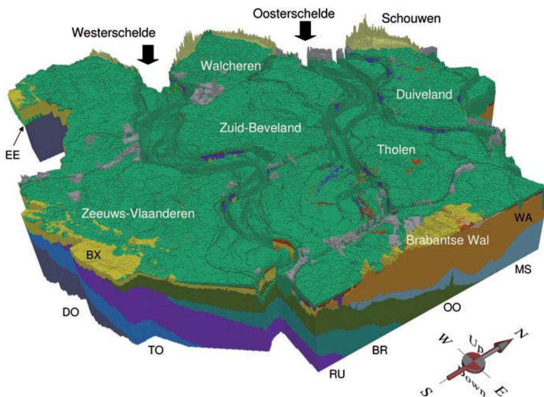
Figure 4.2: The modelled stratigraphical units (volumes). At the surface the Naaldwijk-Walcheren (tidal deposits, green), Naaldwijk Schoorl (coastal dunes, yellow) and anthropogenic deposits (gray) are dominant. The older Formations include: BX: Boxtel, EE: Eem, WA: Waalre, MS: Maassluis, OO: Oosterhout, BR: Breda, RU: Rupel, TO: Tongeren, DO: Dongen (Stafleu et al, 2011).
