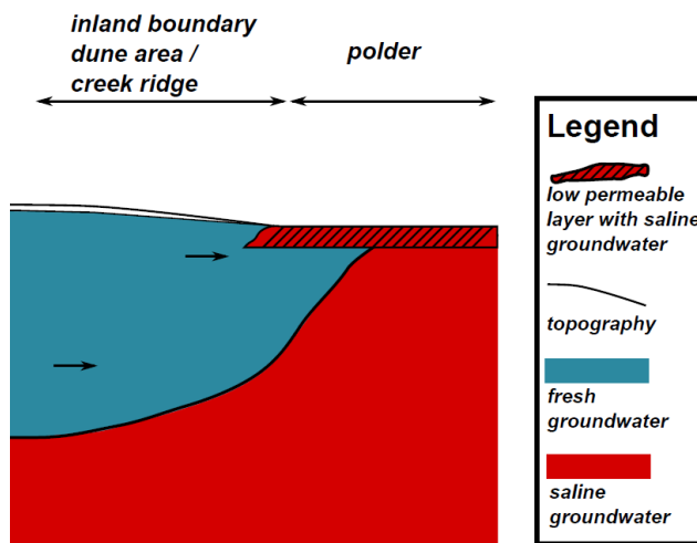
Figure 11.20: Concept of the inversion along the inland boundary of the dune area and next to the creek ridges.
