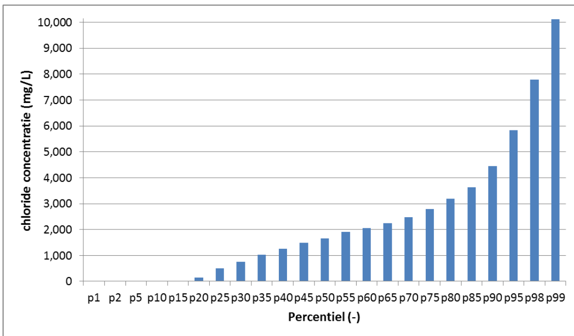
Figure 8.8: Example probability distribution of chloride concentration Midden Zeeland, vlieglijn 310.1
