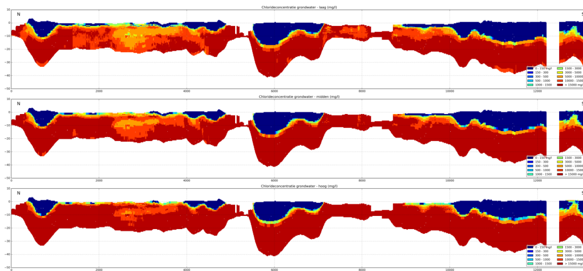
Figure 8.9: 25 th , 50 th and 75 th percentile chloride concentration (top, middle, bottom) for flightline 310.1 (Midden Zeeland)
