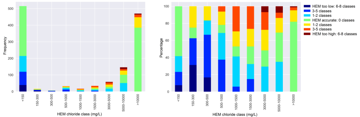
Figure 12.5 Left: validation result per chloride class for FRESHEM result 'middle', absolute number. The green bars represent 59% of the monitoring wells. Right: Validation result per chloride class for the FRESHEM result 'middle', relative per chloride class.
