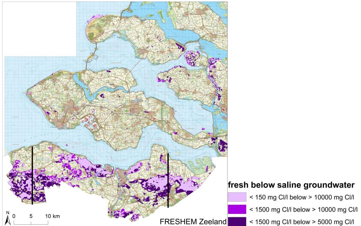
Figure 11.15: Inversions in the 3D chloride concentration model ("middle"). Black lines are the locations of the cross sections of Zeeuws-Vlaanderen in section 11.6.3.4.
