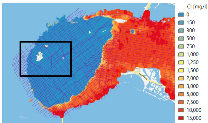
Figure 11.27 P50 of chloride concentration at the western coast of Shouwen Duiveland, at a depth of 19 m below NAP. Flightlines (purple lines) and approximate area indicated in Figure 11.28 and Figure 11.29 (black box).
