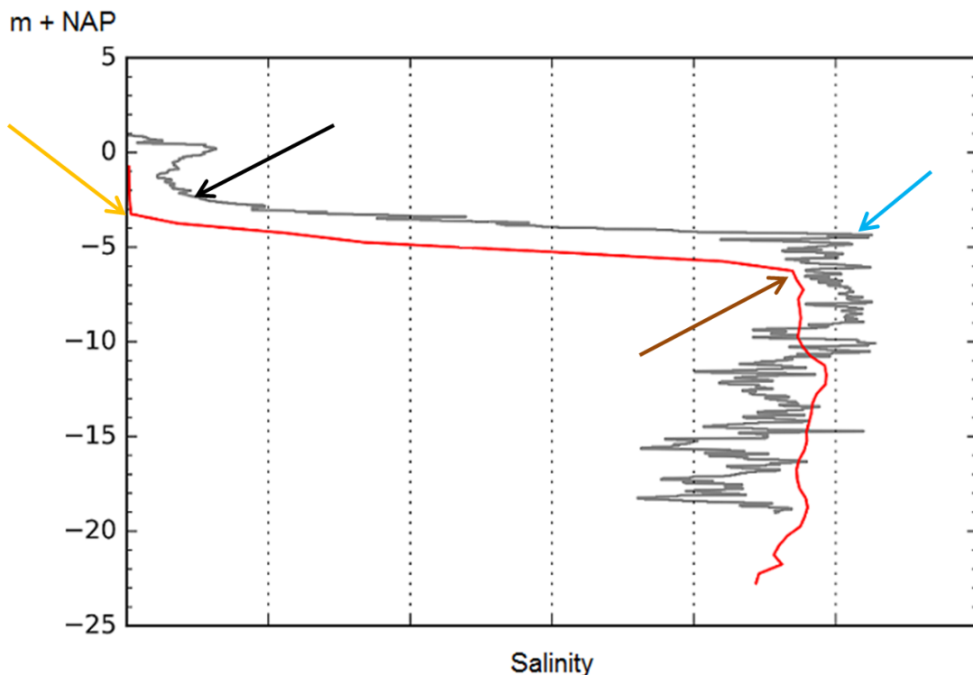
Figure 12.7 Example of visual determination of starting and end depth of fresh-saline mixing zone. The grey line is the EC profile of the ground measurement. The red line is the FRESHEM result for this location. The black arrow indicates the start of the mixing zone according to the ground measurement, at -2.0 m NAP. The orange arrow indicates the start of the mixing zone according to the FRESHEM result, at -3.0 m NAP. The brown arrow indicates the end of the mixing zone according to the FRESHEM result at -6 m NAP, and the blue arrow indicates the end of the mixing zone according to the ground measurement at -4.5 m. The increase and decrease of the EC around 0 m NAP is interpreted as a lithological feature, and not as the presence of saline groundwater; the noisy profile deeper than -4.5 m NAP is also caused by lithology rather than by fluctuating chloride concentrations.
