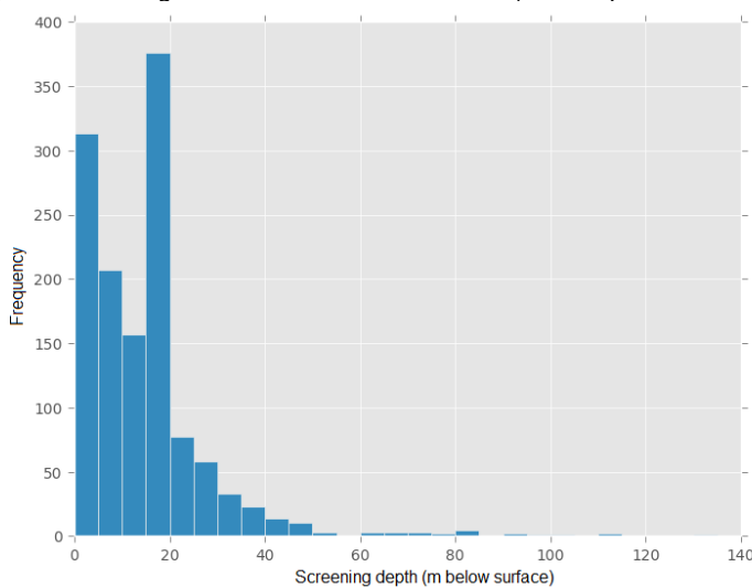
Figure 12.2 Histogram of screening depth of monitoring wells.
