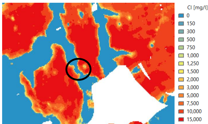
Figure 11.33 Chloride concentration at 6.75 m below NAP, a relatively narrow zone of fresh water is indicated by the black circle.
