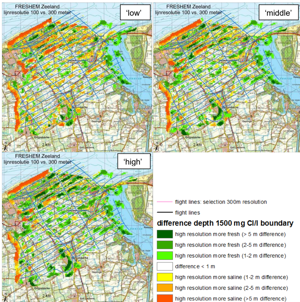
Figure 10.7 Flightline resolution: difference between the 100m and 300m resolution (distance between the flightlines) for a. FRESHEM 'low'; b. FRESHEM 'middle' and c. FRESHEM 'high'.
