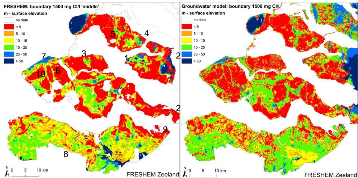
Figure 11.11 a. Depth 1500 mg Cl/l boundary FRESHEM Zeeland 'middle' and b. depth 1500 mg Cl/l boundary Groundwater model (the 'old' map).
