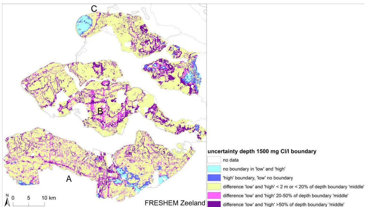
Figure 11.8 Uncertainty depth 1500 mg Cl/l boundary: difference depth 'low' and 'high' as % of depth 'middle'.
