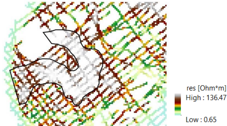
Figure 11.28 Resistivity values at flightlines at a depth of 19 m below NAP. Indicated is the interpretation of a relatively high resistivity area.
