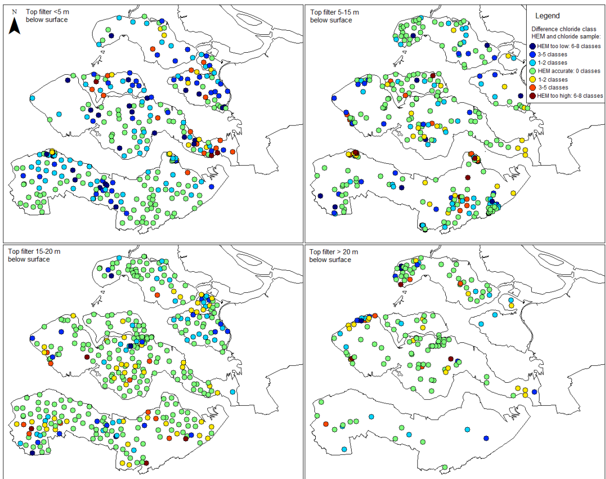
Figure 12.6: Validation chloride results for p50 FRESHEM result separated per filter depth.
