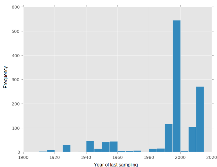
Figure 12.3 Year of last sampling of the monitoring wells. Some monitoring wells are no longer sampled; many have last been sampled in the second half of the decade 1990-2000.
