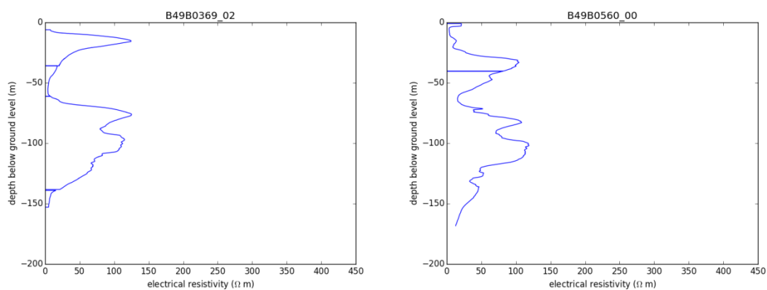
Figure 11.24: Borehole logging measurements East of De Eendracht / Schelde-Rijnkanaal (see Figure 11.25). Both measurements indicate fresh groundwater between ~60 m below ground level and ~120 m below ground level. Between ~30-40 m below ground level and ~50-60 m below ground level the groundwater at some depth is probably saline or brackish. This is probably also the case close to the surface.
