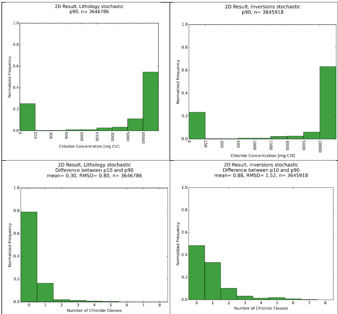
Figure 10.2: Histograms of p10, p50, p90 and number of classes difference between p10 and p90, for the 2D result with the stochastic variable lithology and different inversion methods respectively.
