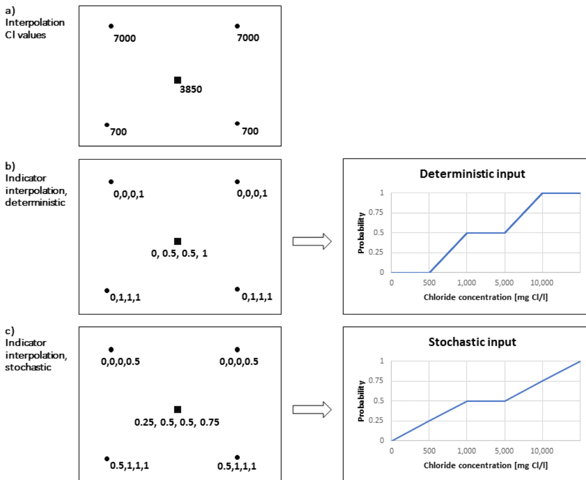
Figure 9.2: Simple interpolation examples: a) 'normal', b) indicator, c) indicator with stochastic input.
