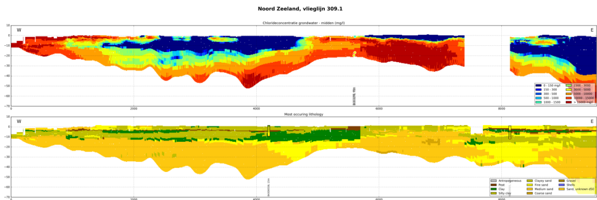
Figure 11.21: Inversion on Sint Philipsland (left) East of the Schelde-Rijnkanaal (right) in flightline 309.1.
