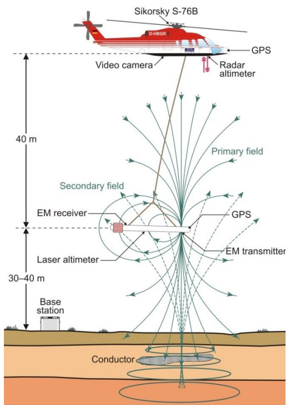
Figure 5.2: Sketch of BGR's airborne geophysical system.
