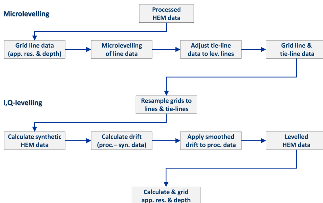
Figure 6.2: Levelling procedure.
