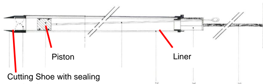
Figure B7: Schematic representation of the Beaker Sampler (adopted from Beeker, 1989).
