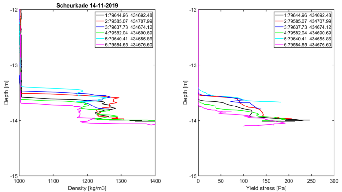
Figure A144. Fluid mud detection at the Scheurkade on 14-11-2019: density (left) and yield stress (right) profiles
