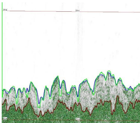
Figure A50. Fluid mud detection at the 8e Petroleumhaven on 27-01-2020: line 3. Blue level – water-mud interface, red level – sharp density contrast in seismic data, green level – multibeam level.
