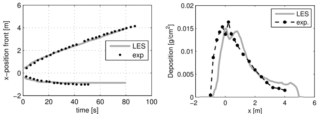
Figure D4. Asymmetric spreading of a density current at a bed with ambient current, position front (left) and final deposition at the bed (right).
