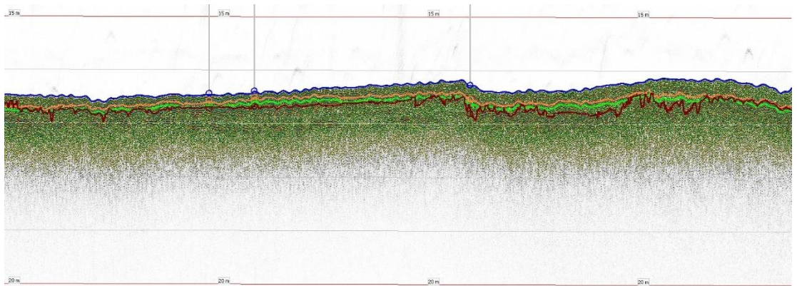
Figure A34. Fluid mud detection at KTM kade on 13-11-2019: line 2 (continued). Blue level – water-mud interface, red level – sharp density contrast in seismic data, orange level – 1.2 kg/l (density) level, green level – 100 Pa (Bingham yield stress) level.
