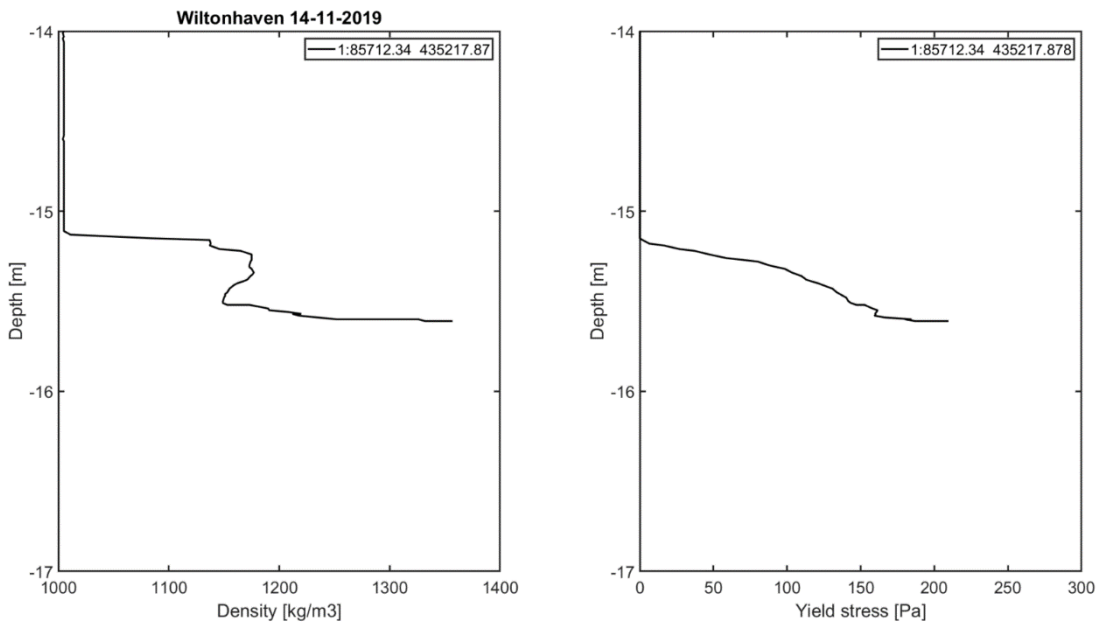
Figure A146. Fluid mud detection at the Wiltonhaven on 14-11-2019: density (left) and yield stress (right) profiles
