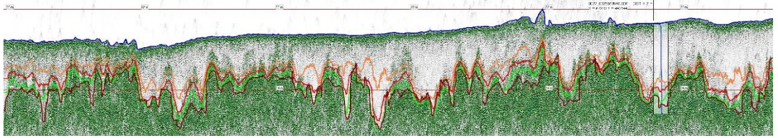
Figure A124. Fluid mud detection at the Calandkanaal on 25-03-2020: line Calandkanaal 6_0325075525. Blue level – water-mud interface, dark red level – sharp density contrast in seismic data, green level – 1.2 kg/l (density), bright red level – 1.17 kg/l (density) level, orange level – 1.15 kg/l (density) level. Blue vertical line shows density profiles
