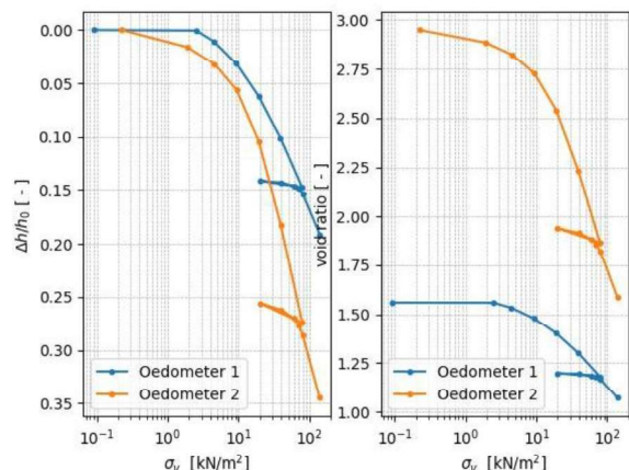
Figure 3. 24h compression curves, left) stress vs strain right) stress vs void ratio, e.
