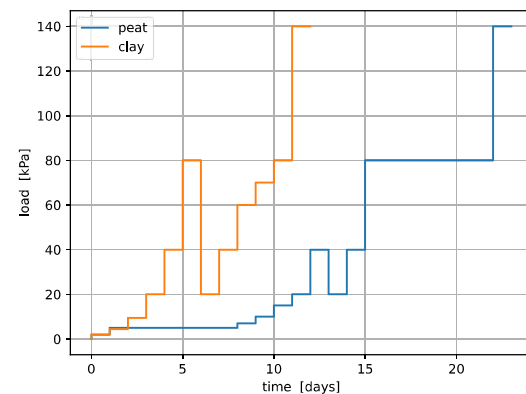
Figure 1. Applied loading schemes.
