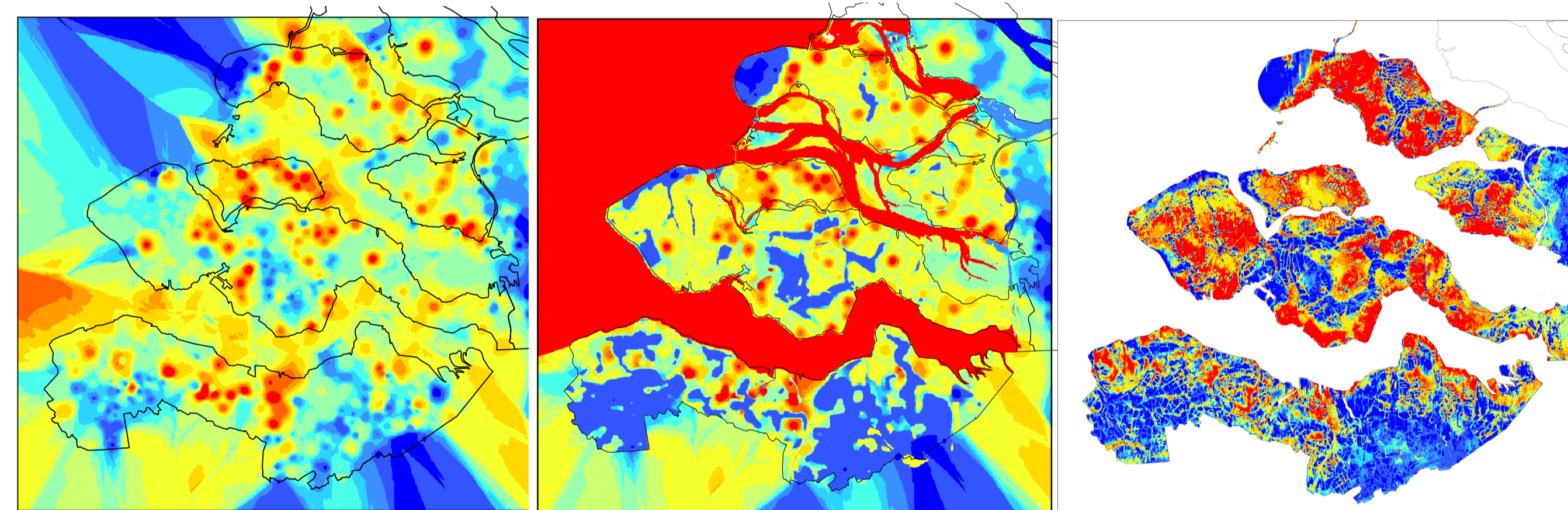
Fig. 5: Chloride concentration groundwater at -6.5 m NAP in three steps: a. interpolating data; b. including interfaces and c. model result 2010.
