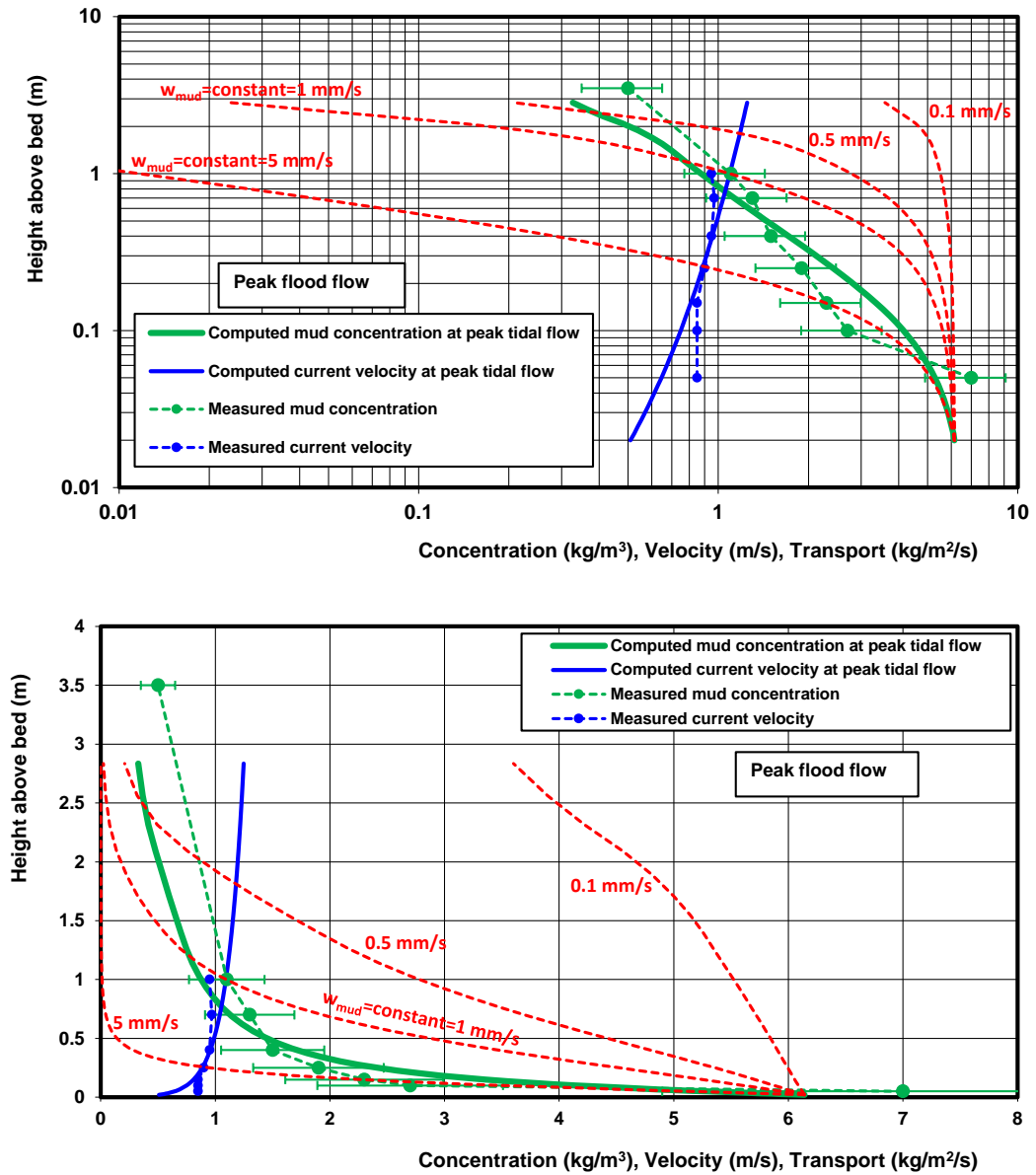
Figure 27 Effect of constant settling velocity on computed concentration profile at peak flood flow; Day 3 (Upper: logarithmic axis; Lower: linear axis)
