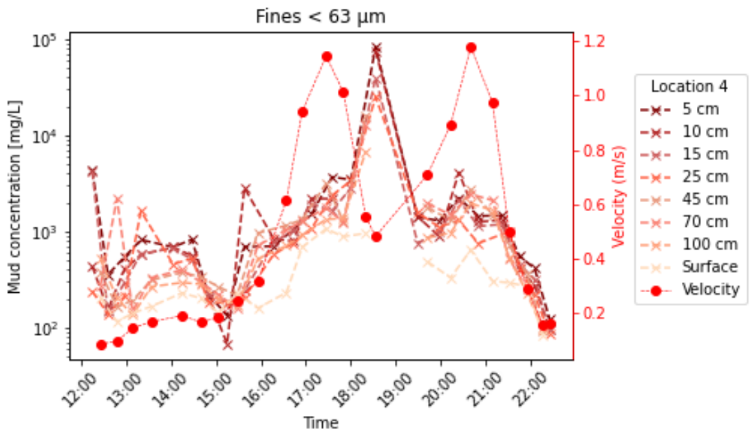
Figure A 29 Mud concentrations (fines < 63 μm) at various elevations above the bed and depth-averaged current velocity over tidal cycle; Day 4; 15 June 2022
