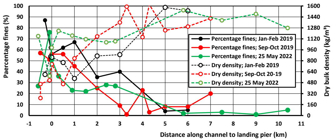
Figure 7 Percentage of fines < 63 \mu\text{m} and dry bulk density; Holwerd ferry channel.
