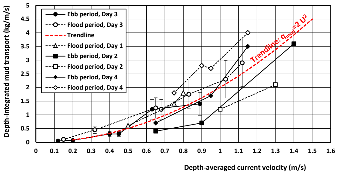
Figure 18 Depth-integrated mud transport as function depth-averaged velocity near Holwerd
