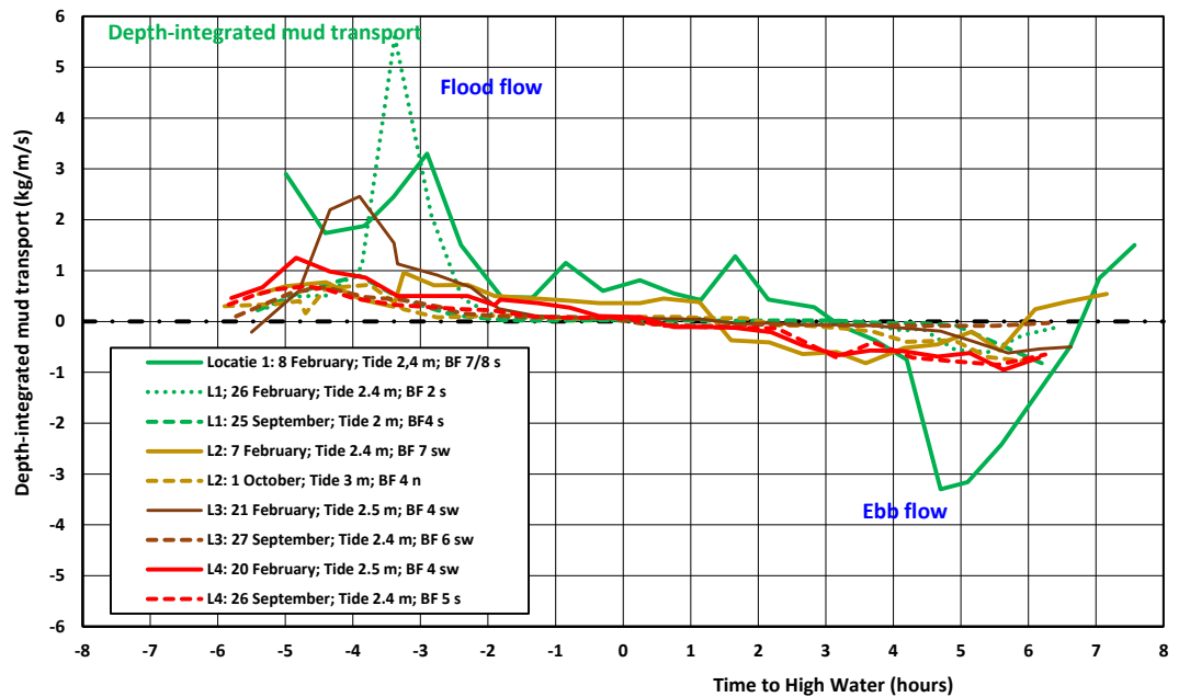
Figure B5 Depth-integrated mud transport over tidal cycle, location 1,2,3,4; ferry channel Holwerd
