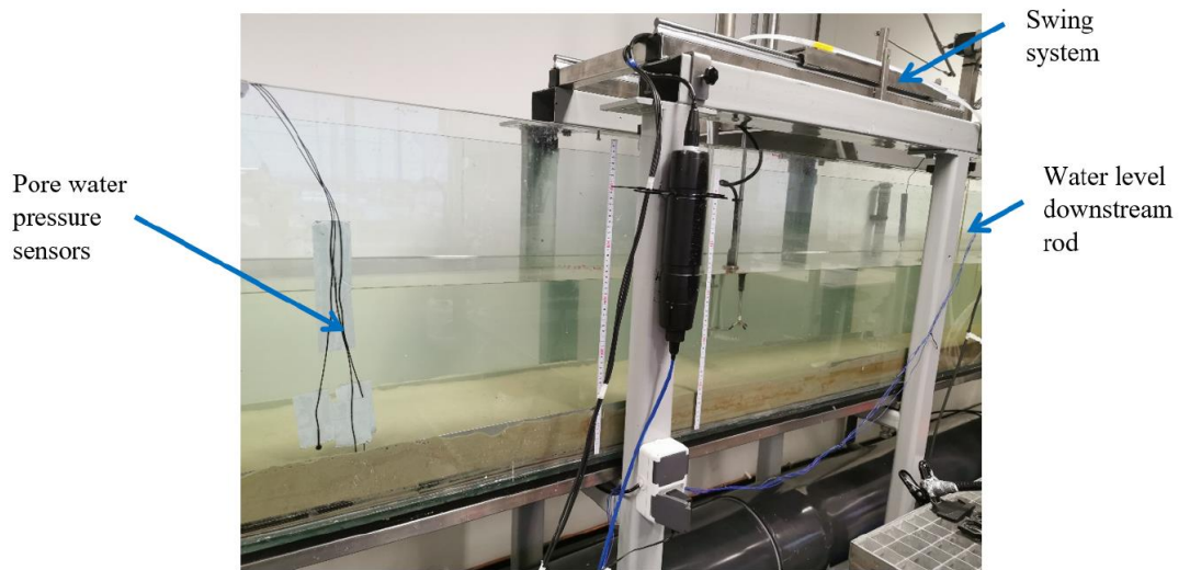
Figure 3.2.2 Instrumentation installed on the current-wave flume
