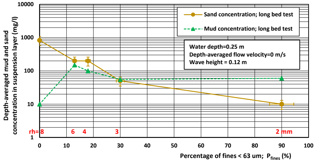
Figure 4.4.4 Depth-averaged sand and mud concentrations as function of percentage of fines <63\ \mu\text{m} ; waves alone ( H=0.12\text{ m} ; water depth= 0.25\text{ m} ). R_h = Ripple height in millimetres.
