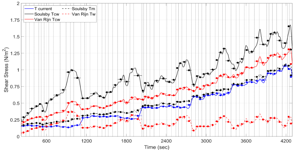
Figure B. 14: Computed bed-shear stress as function of time; undisturbed sample BA-APP. T current = current-related bed-shear stress; Soulsby Tcw = maximum bed-shear stress current+waves according to method of Soulsby; Van Rijn Tcw = time-averaged bed-shear stress current+waves according to method of Soulsby; Van Rijn Tcw = time-averaged bed-shear stress current+waves according to method of Van Rijn; Soulsby Tm = time-averaged bed-shear current+waves according to method of Soulsby; Van Rijn Tw = time-averaged bed-shear stress waves according to method of Van Rijn.
