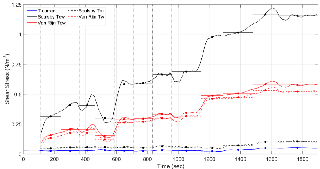
Figure B. 2: Computed bed-shear stress as function of time; remoulded sample BA-4 ( u_m=0.1 m/s). T current = current-related bed-shear stress; Soulsby Tcw = maximum bed-shear stress current+waves according to method of Soulsby; Van Rijn Tcw = time-averaged bed-shear stress current+waves according to method of Soulsby; Van Rijn Tcw = time-averaged bed-shear stress current+waves according to method of Van Rijn; Soulsby Tm = time-averaged bed-shear current+waves according to method of Soulsby; Van Rijn Tw = time-averaged bed-shear stress waves according to method of Van Rijn.
