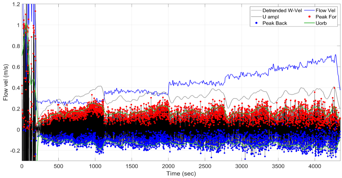
Figure B. 13: Measured velocity signal as function of time; sample BA-APP. Detrende W-vel = orbital velocity minus time-averaged velocity; Flow vel = time-averaged flow velocity; U amp = maximum velocity; Peak Back = maximum backward orbital velocity; Peak For = maximum forward orbital velocity; Uorb = smoothed peak orbital velocity.
