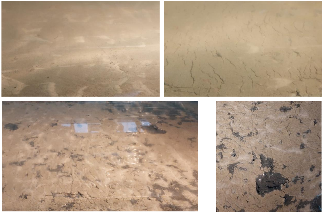
Figure C. 4: Upper left: bed before Test E; Upper right: bed with darker mud cracks/craters during Test E-2 (H=12 cm.) Lower: bed after test E-2 with mud/silt top layer, sand spots, mud craters (30 mm; 10 mm deep)
