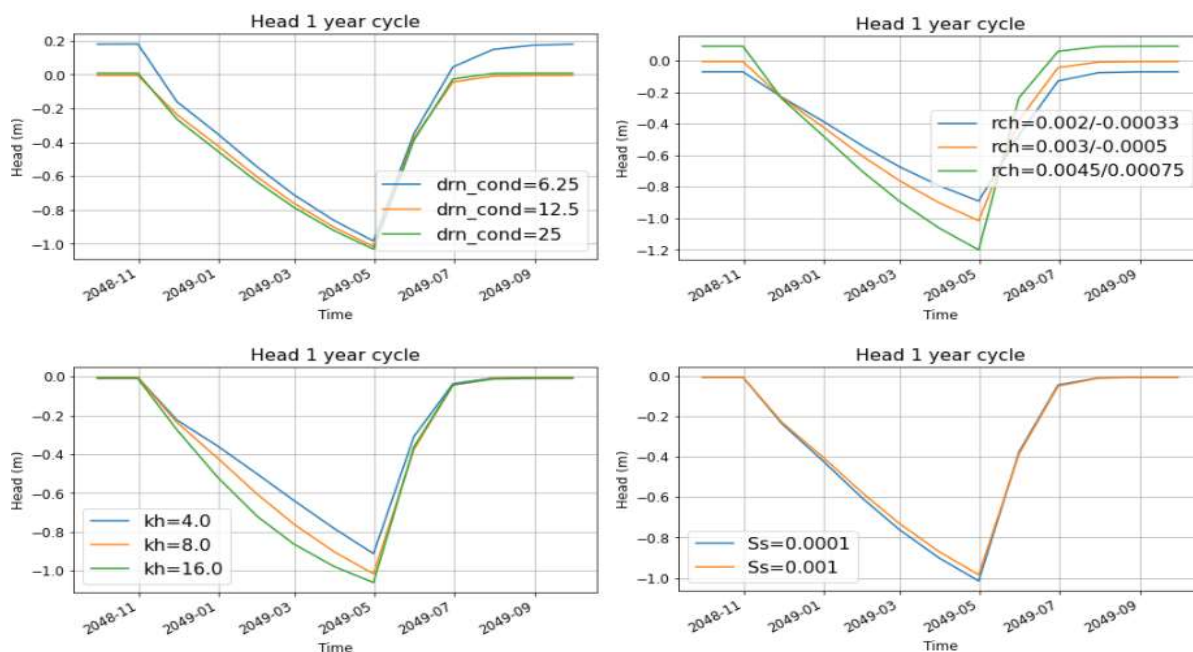
Figure 19. One-year cycle of the hydraulic head at (0,0) layer 1, showing variation in drainage conductance (upper left), recharge rate (upper rate), horizontal conductivity (bottom left) and specific storage (bottom right).
