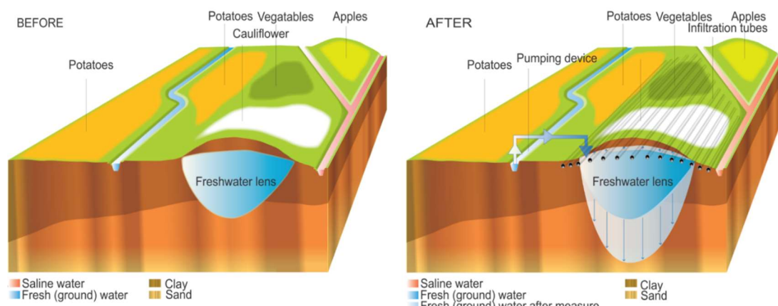
Figure 2. Conceptual visualization of an ASR system (Pauw et al., 2015).
