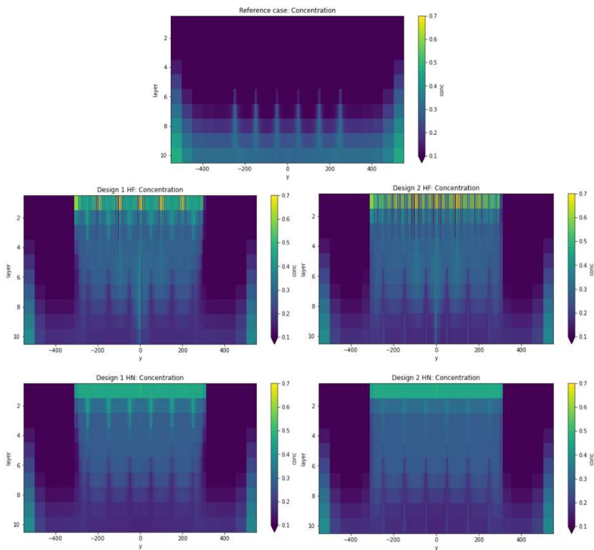
Figure 33. Groundwater concentration at transect x=0 for the scenarios HF and HN of ASR design 1 (left) and 2 (right) at the end of the dry period.
