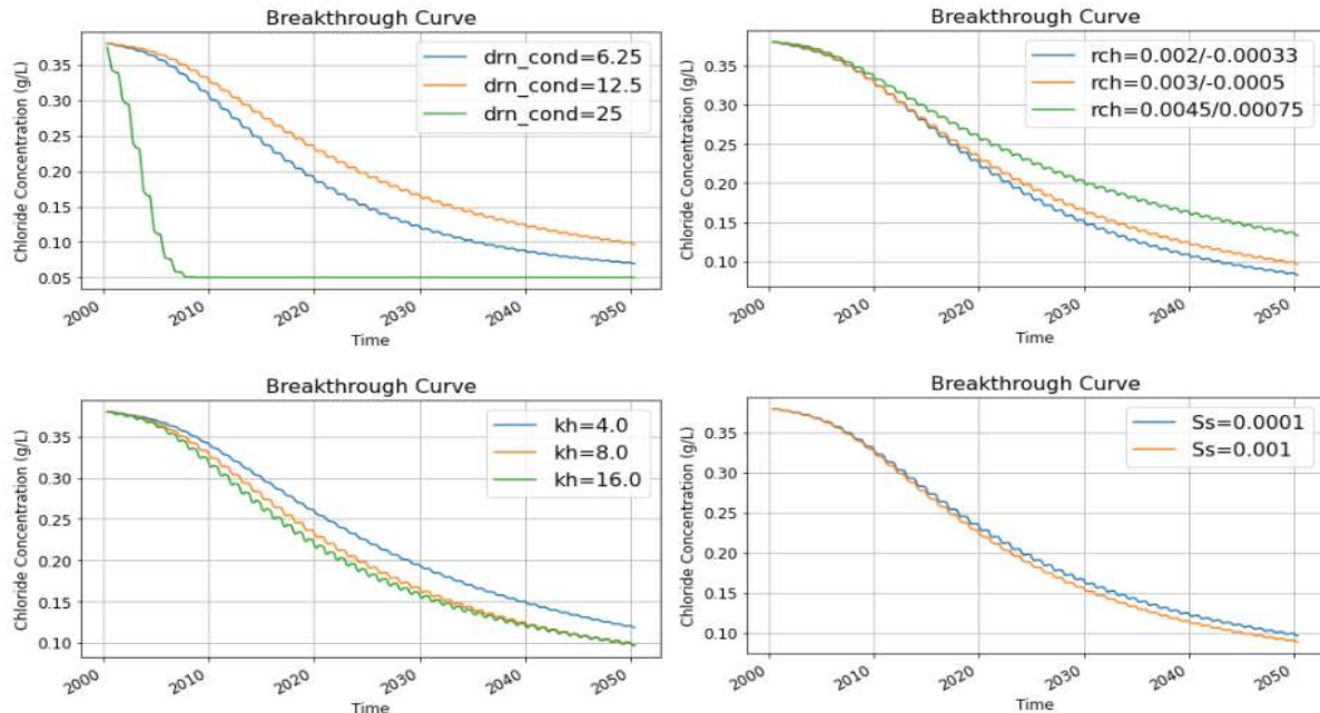
Figure 18. Breakthrough curves at (U,U) layer 5, showing variation in drainage conductance (upper left), recharge rate (upper rate), horizontal conductivity (bottom left) and specific storage (bottom right).
