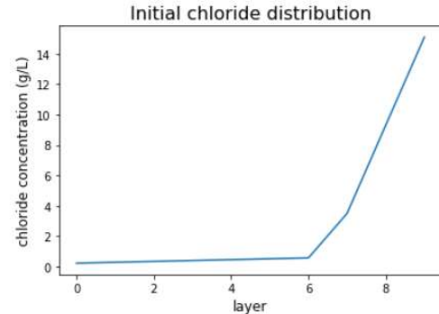
Figure 25. Initial chloride distribution when adding a layer of saltwater ( 15 \text{ g/L} ) to the model.
