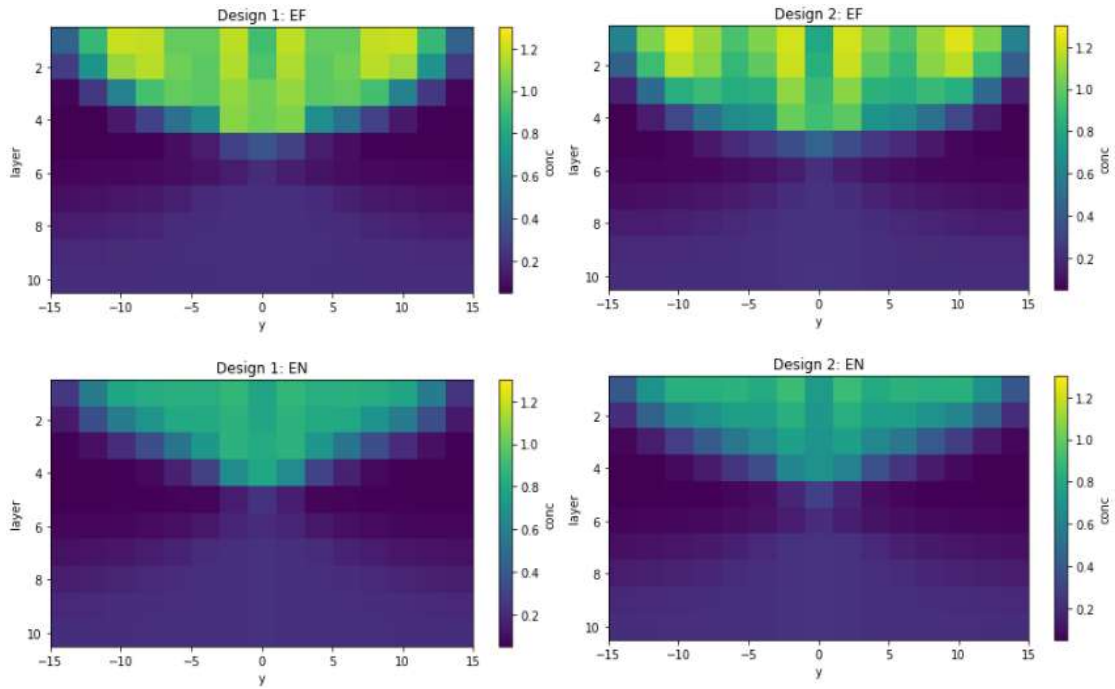
Figure 41. The concentration at the end of the dry period for the transect at x=0 for design 1 (left) and design 2 (right) for 'extreme' scenarios.
