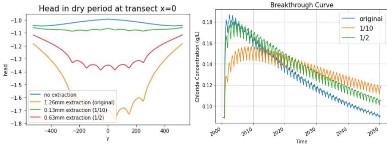
Figure 29. Hydraulic head at transect x=0 at the end of the dry period showing the effect of various groundwater extraction rates (left). Breakthrough curve at location of extraction well showing the effect of various groundwater extraction rates on the concentration in the well (right).
