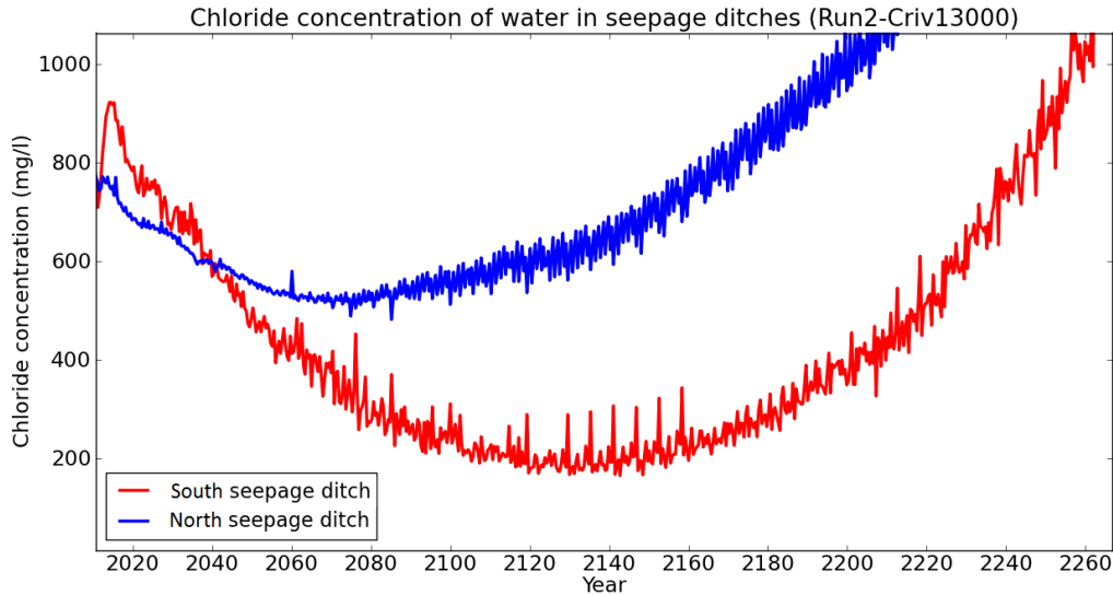
Figure 4.5 Chloride concentration in the seepage ditches in scenario Criv13000 .
