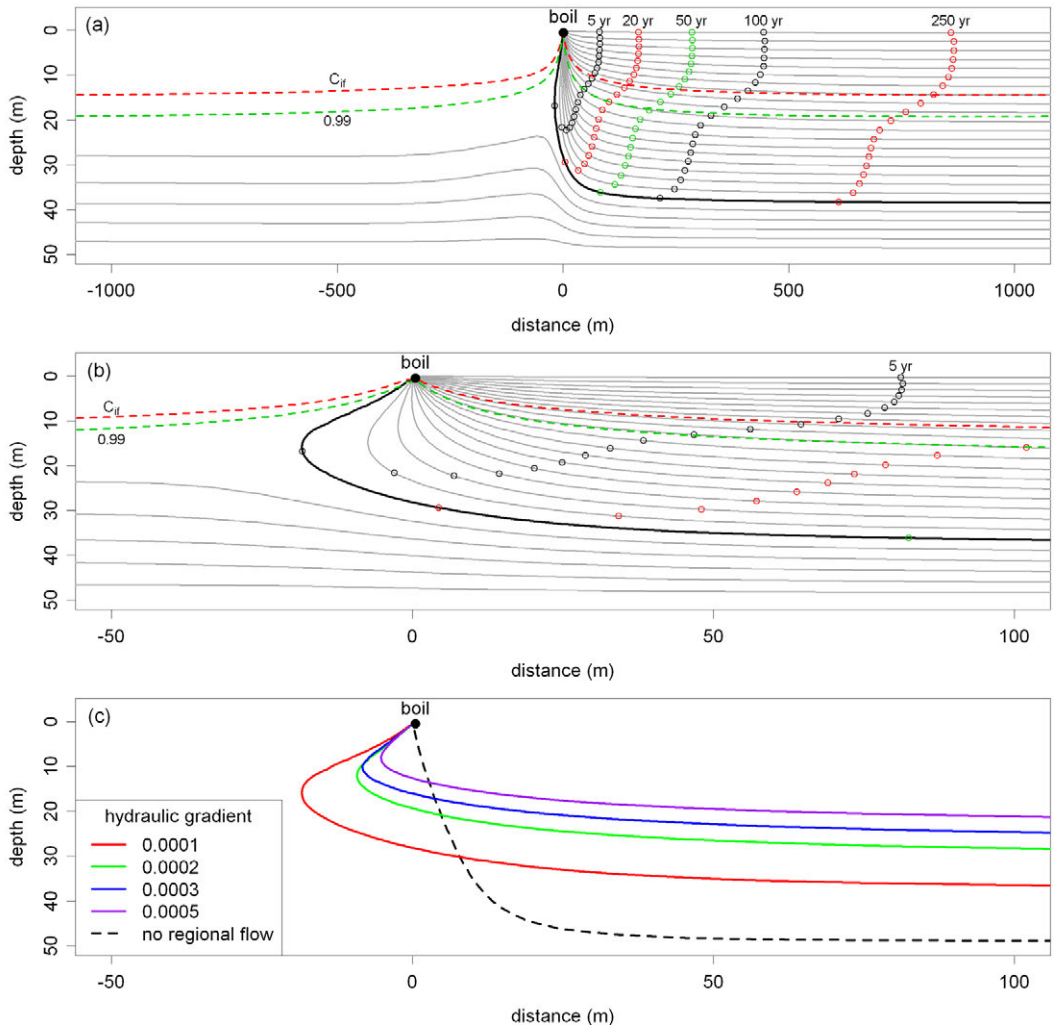
Fig. 4.10. (a) Streamlines towards the boil with travel times to the boil (in yr) for the case with regional flow (hydraulic gradient = 0.0001). The coloured points at the streamlines indicate the travel time to the boil. The relative salinity contours of 0.50 ( C_{ij} ) and 0.99 (bottom transition zone) are indicated as well. (b) Same as Fig. 4.10a but zoomed in. (c) Dividing streamlines for the regional flow cases with different hydraulic gradients and the reference case without regional flow.
