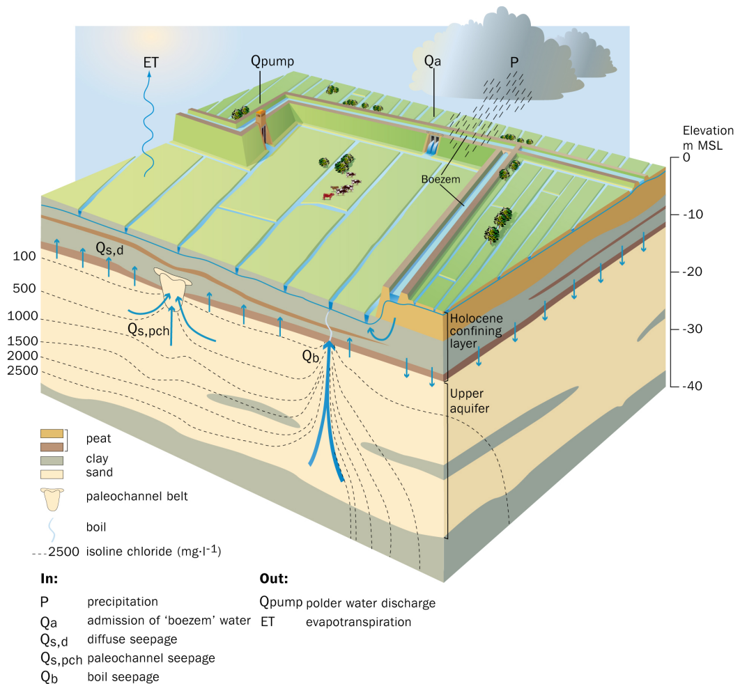
Fig. 3.1. The hydrogeology and water and salt fluxes in a lowland polder catchment area. Upward groundwater seepage from the upper aquifer can be divided into three different types according to De Louw et al. (2010): diffuse-, paleochannel-, and boil seepage.
