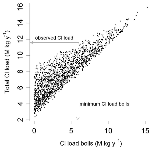
Fig. 2.11 Scatter diagram of calculated chloride load via boils versus calculated total chloride load in the Noordplaspolder.
