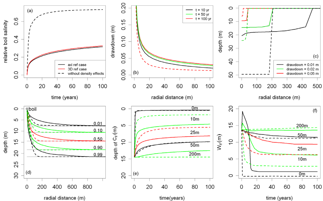
Fig. 4.5. Model results of axisymmetric reference case with density effects (full lines) and without density effects (dotted lines): (a) boil salinity with time, (b) freshwater head drawdown for different simulation times, (c) freshwater head drawdown contours (after 100 yr), (d) upconing of different relative salinity contours (after 100 yr); grey lines indicate the initial position of the salinity contours, (e) change of C_{if} and (f) W_{if} with time at different distance from the boil.
