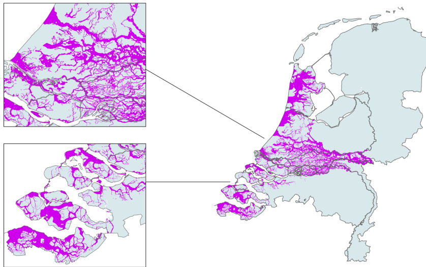
Fig. 1.4 (a) A general picture of the composition of the Holocene confining layer in western Netherlands with sandy paleochannel belts cutting through the lower part of the Holocene confining layer. (b) The location of sandy paleochannels in western Netherlands (Stafleu et al. , 2013) and the south-western delta (Stafleu et al. , 2011). Maps of paleochannels in the northern coastal area were not yet available.
