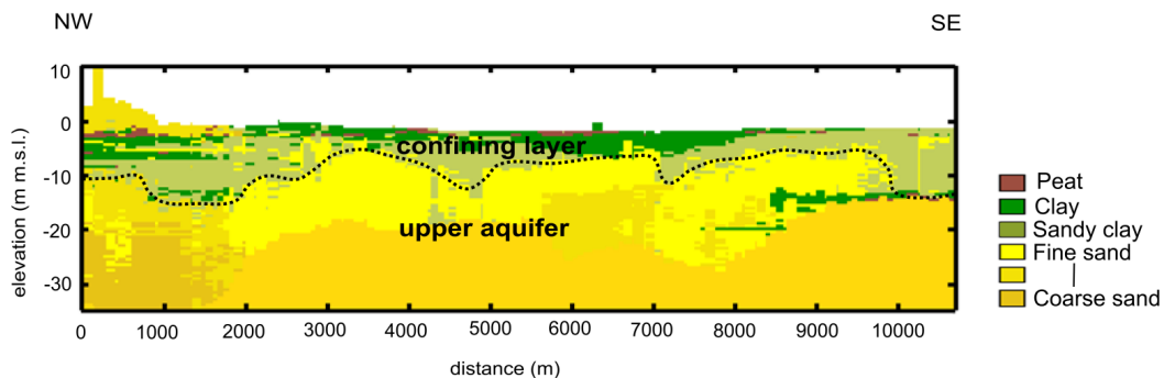
Fig. 5.3. A NW-SE lithological cross-section of the island of Schouwen-Duivenland (see Fig. 5.4 for location of cross-section). The cross-section is derived from a detailed 3D geological model of Zeeland based on 5 drillings per 1 km 2 that were classified into geological units (GeoTOP, Stafleu et al. , 2011).
