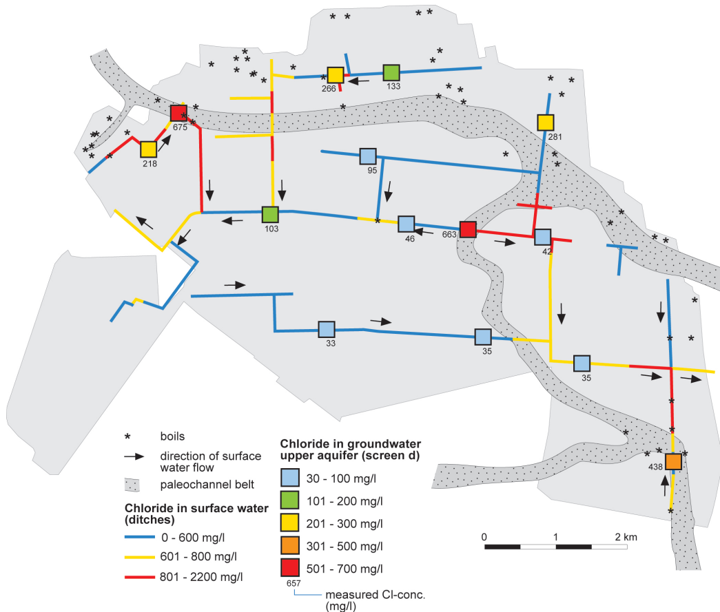
Fig. 2.6. Chloride monitoring results (mg/l) for the Noordplaspolder: surface water in August 1999 (sampling interval 250 m) and groundwater at the top of the upper aquifer, screen d (average of April and September 1999). The mapped boils and location of the paleochannel belts in the Holocene confining layer are indicated.
