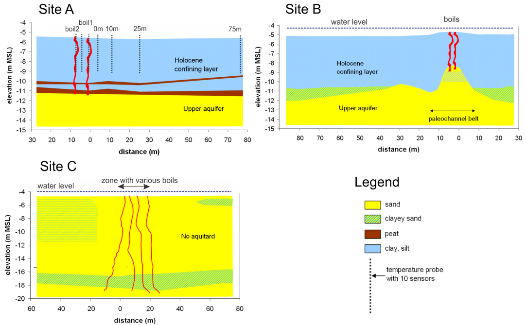
Fig. 7.3. The hydrogeological schematization of the three boil locations. The location of the temperature probes for site B and C are similar to those of site A
