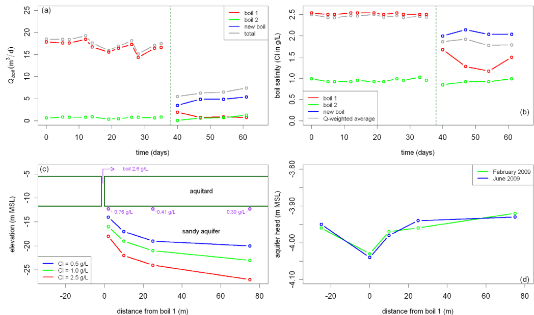
Fig. 4.4. Field measurements of boil site A. (a) Q_{boil} and (b) boil salinity with time; the boil sealing experiment is indicated by the dotted green lines, (c) isochlors of Cl concentration from ECPT measurements and groundwater Cl concentration (in purple), (d) equivalent freshwater aquifer heads.
