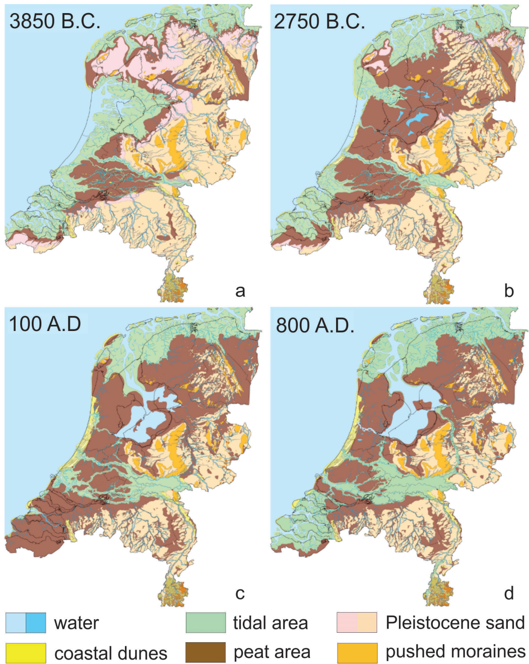
Fig. 1.2. The paleogeographical development of the Netherlands in four phases: (a) 3850 B.C., (b) 2750 B.C., (c) 100 A.D., (d) 800 A.D. (Vos et al. , 2011).
