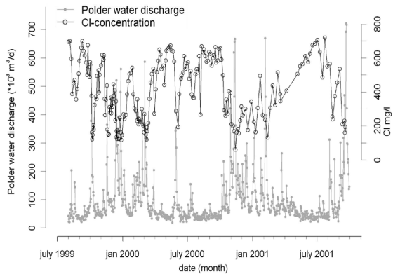
Fig. 2.5. Daily discharge volume and chloride concentration of water pumped out of the polder over period July 1999 – September 2001.
